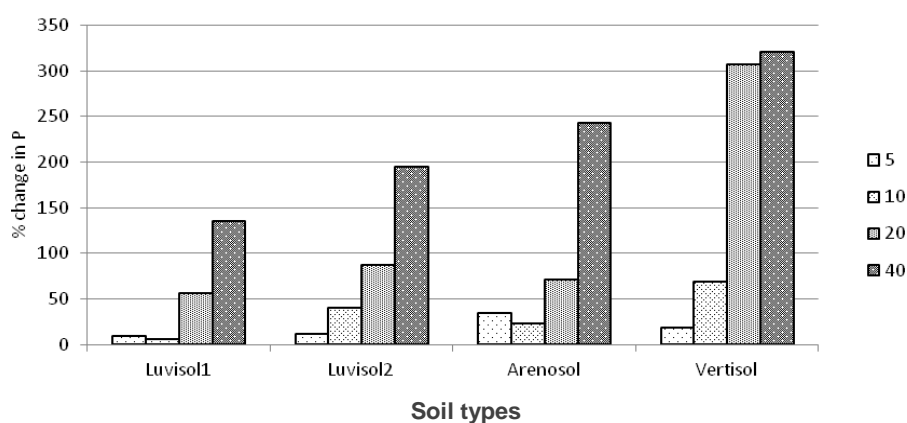
Figure 4. Percentage change in phosphorus in soils three months after sludge addition.
