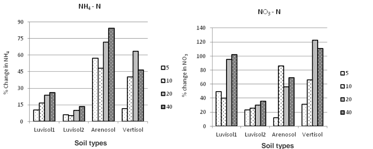
Figure 5. Percentage change in NO 3 - N and NH 4 - N in all soils three months after sludge addition.
