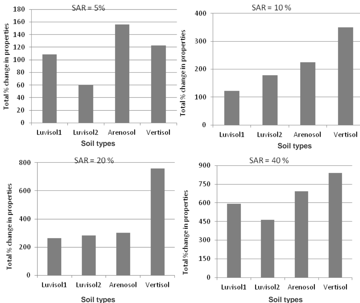
Figure 7. Percentage change in soil properties at different SAR.
