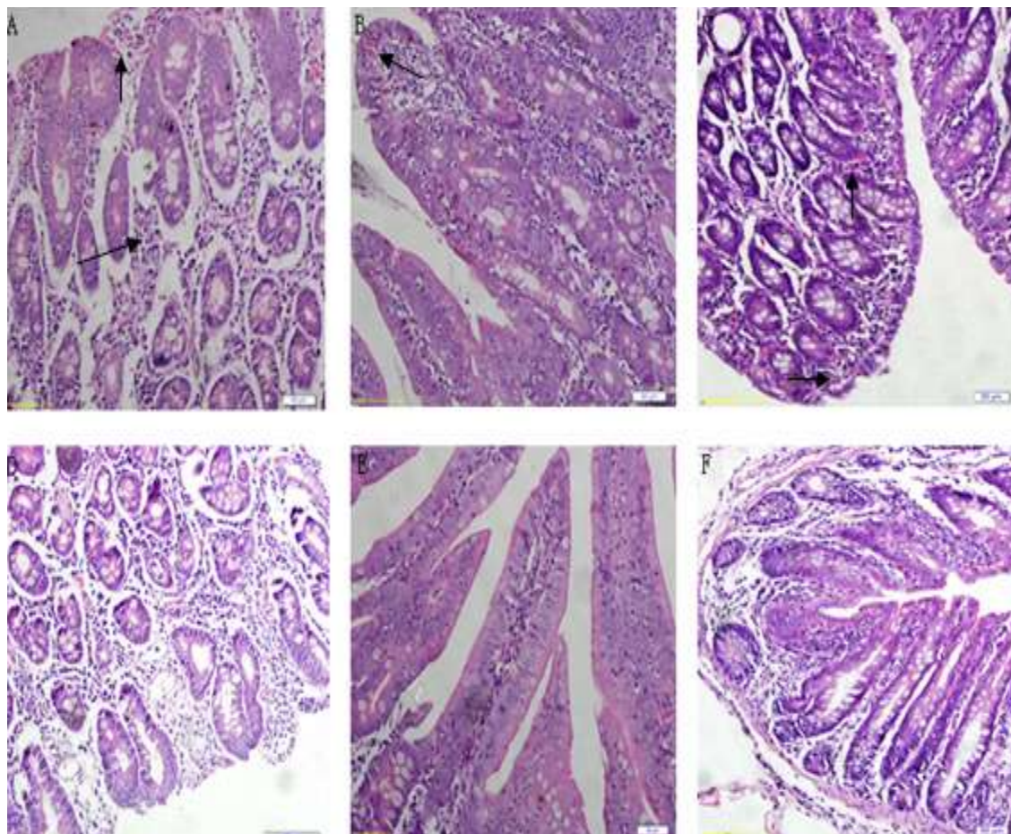
Figure 1. Representative H and E-stained histological sections of stomach, small intestine and large intestine from the diarrheic group (Figure 1A, B and C) with slides D, E and F providing normal comparisons respectively. Bar = 100 \mu m.
