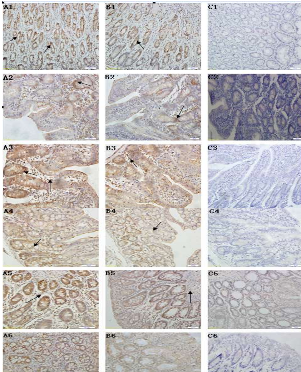
Figure 2. Immunolocalization of PAR-2 in piglet gastrointestinal tract mucosa from healthy and diarrhea piglets using immunohistochemistry. Strong staining was exhibited in the gastric gland of the stomach mucosa (A1), duodenum mucosa (A2), jejunum mucosa (A3), ileum mucosa (A4), cecum mucosa (A5) and colon mucosa (A6) compared to control cells (slides C1-C6 respectively) and healthy cells (B1-B6 respectively). Arrows indicate positive staining for PAR-2, reference bar = 50 \mu m.
