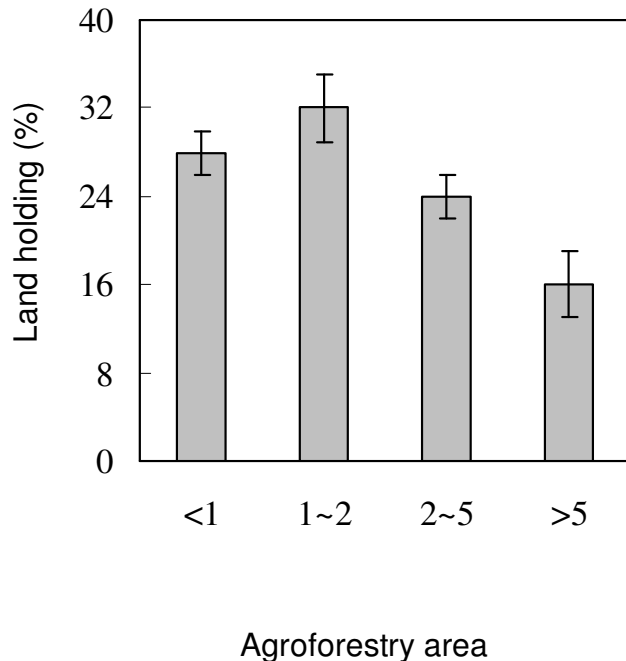
Figure 1. Distribution of landholdings under agroforestry.
