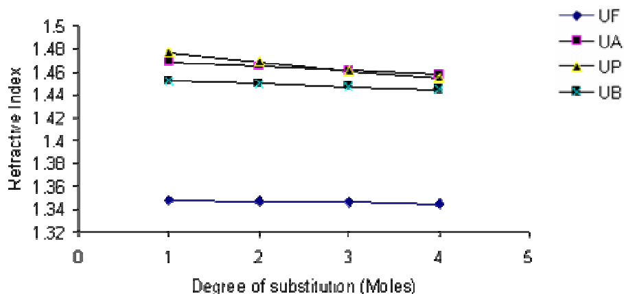
Figure 7. Effect of aldehydic group and degree of substitution on the refractive index of amino resins. UF = Formaldehyde, UA = urea acetaldehyde, UP = urea proparaldehyde and UB = urea butaldehyde.
