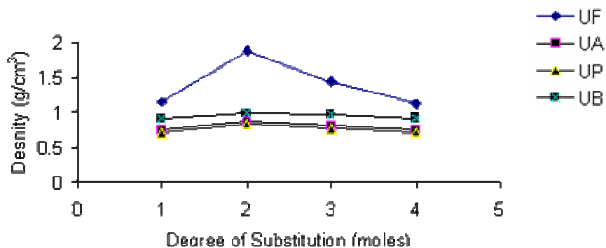
Figure 6. Effect of aldehydic group and degree of substitution on the density of amino resins. UF = Formaldehyde, UA = urea acetaldehyde, UP = urea proparaldehyde and UB = urea butaldehyde.
