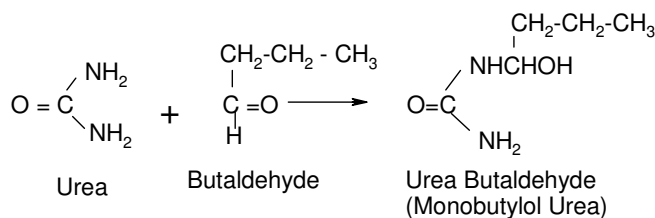
d. Reaction of urea and butaldehyde.
