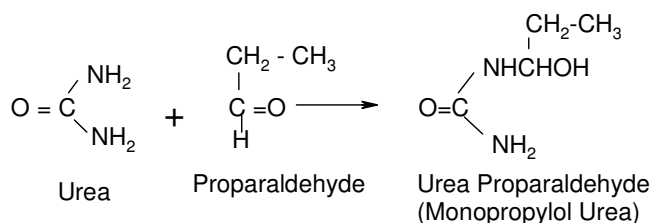
c. Reaction of urea and propionaldehyde.
