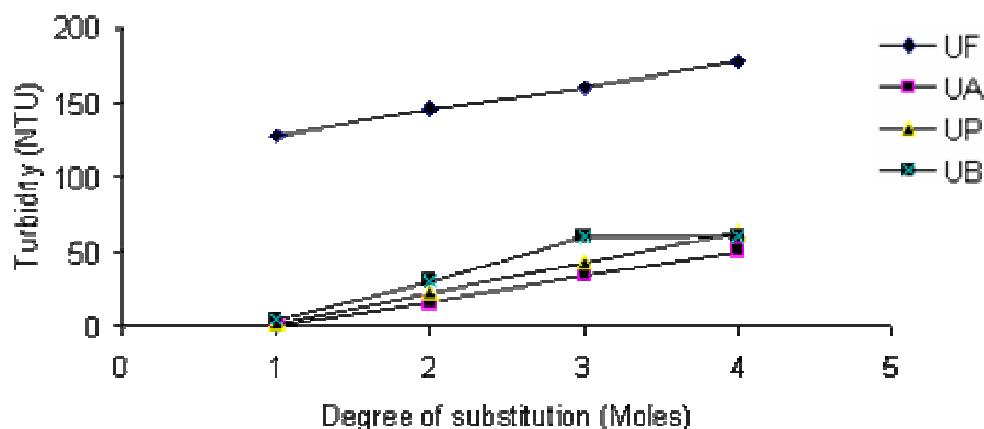
Figure 5. Effect of aldehydic group and degree of substitution on the turbidity of amino resins. UF = Formaldehyde, UA = urea acetaldehyde, UP = urea proparaldehyde and UB = urea butaldehyde.
