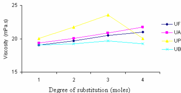
Figure 3. Effect of aldehydic group and degree of substitution on the viscosity of amino resins. UF = Formaldehyde, UA = urea acetaldehyde, UP = urea proparaldehyde and UB = urea butaldehyde.
