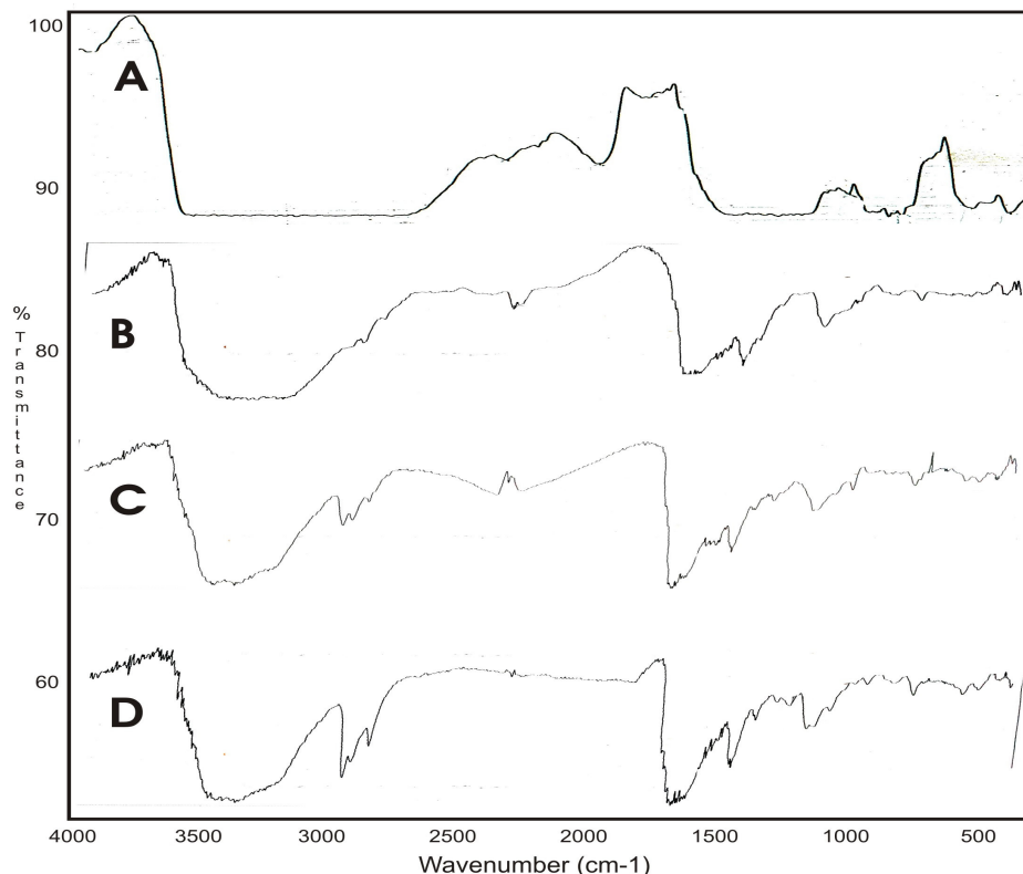
Figure 2. IR Spectra of (A) formaldehyde, (B) urea acetaldehyde (C) urea proparaldehyde and (D) urea butaldehyde.
