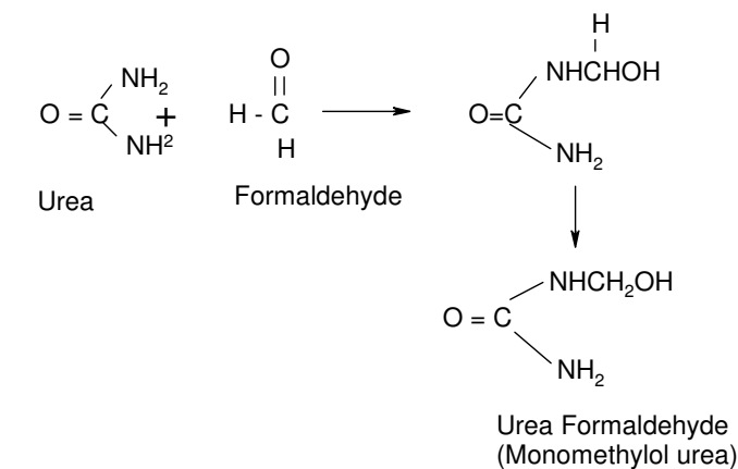
a. Reaction of urea and formaldehyde.
