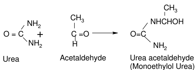
b. Reaction of urea and acetaldehyde.
