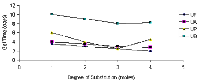
Figure 4. Effect of aldehydic group and degree of substitution on the gel time of amino resins. UF = Formaldehyde, UA = urea acetaldehyde, UP = urea proparaldehyde and UB = urea butaldehyde.
