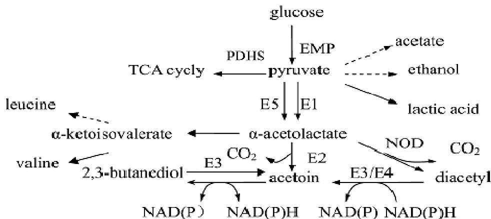
Figure 6. Biosynthetic pathway of acetoin in bacteria. EMP, Embden-Meyerhof-pathway; TCA, tricarboxylic acid cycle; NAD(P), oxidized coenzyme I (II); NAD(P)H, reduced coenzyme I (II); PDHS, pyruvate dehydrogenase system; NOD, nonenzymatic oxidative decarboxylation; E1, catabolic \alpha -Acetolactate synthase; E2, \alpha -acetolactate decarboxylase; E3, 2,3-butanediol dehydrogenase; E4, diacetyl reductase; E5, anabolic \alpha -acetolactate synthase.
