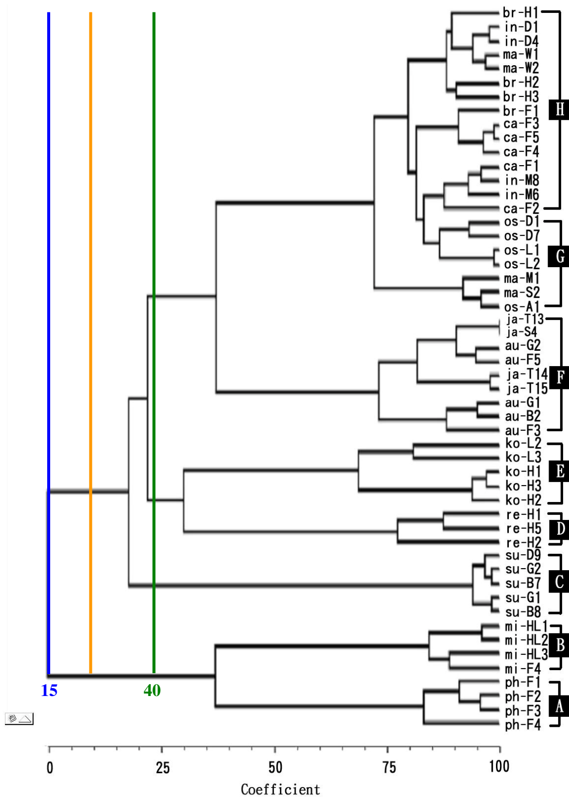
Figure 2. UPGMA dendrogram based on a phenetic analysis of leaf morphology (Cluster A: C. philippinense ; B: C. micranthum ; C: C. subavenium ; D: C. reticulatum ; E: C. kotoense ; F: C. C. pseudomelastoma and C. japonicum ; G: C. osmophloeum ; H: C. insularimontanum , C. macrostemon , C. camphora and C. brevipedunculatum ; refer to Table 1 for OTU codes).
