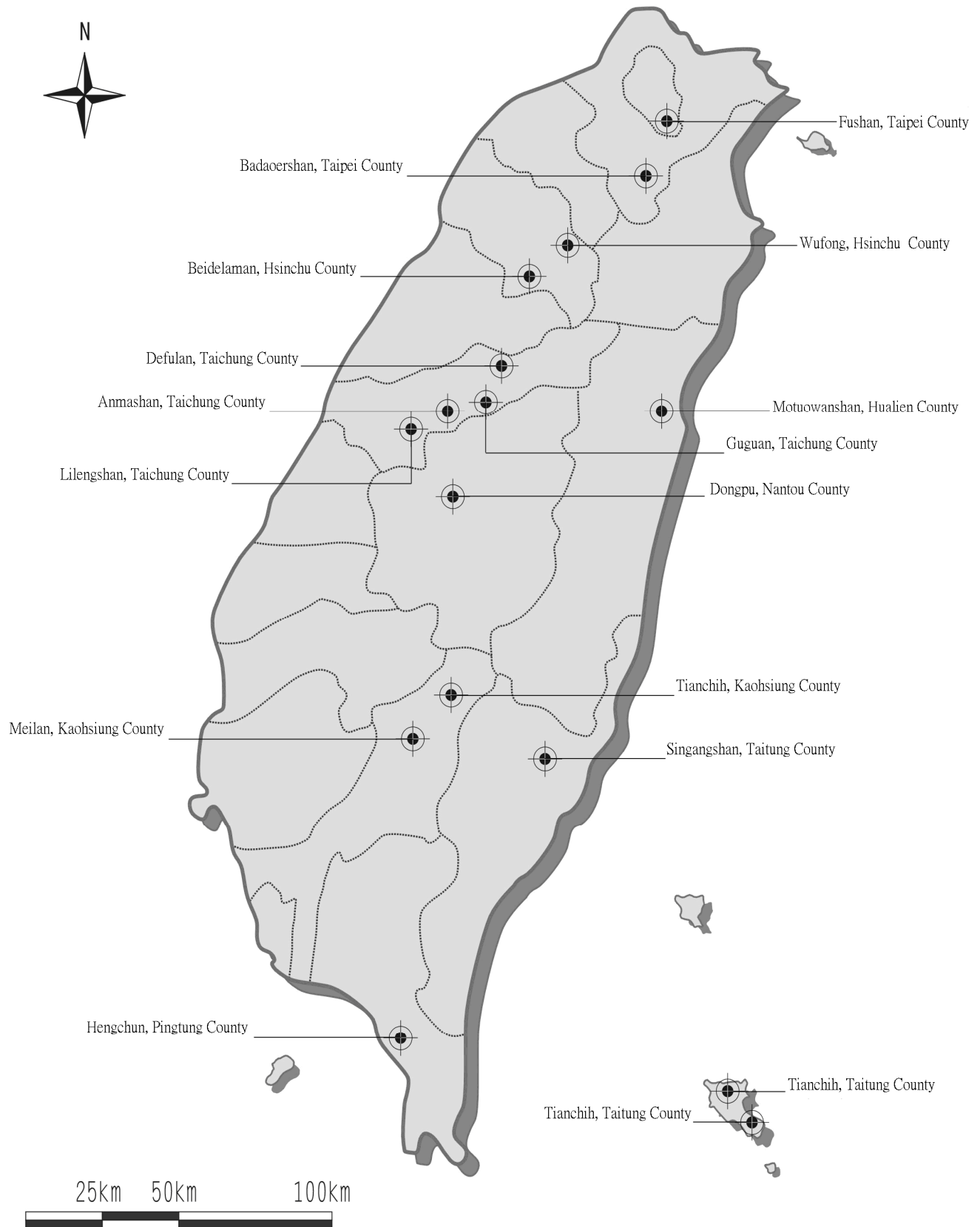
Figure 1. Taiwanese collection sites of Cinnamomum spp.
