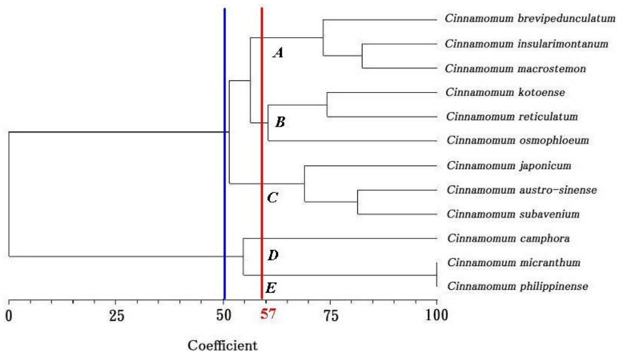
Figure 3. UPGMA dendrogram based on ISSR data. Two clusters are grouped at a distance coefficient of 50 (corresponding to sections Camphora and Cinnamomum ). Five clusters are grouped at a distance coefficient of 57.
