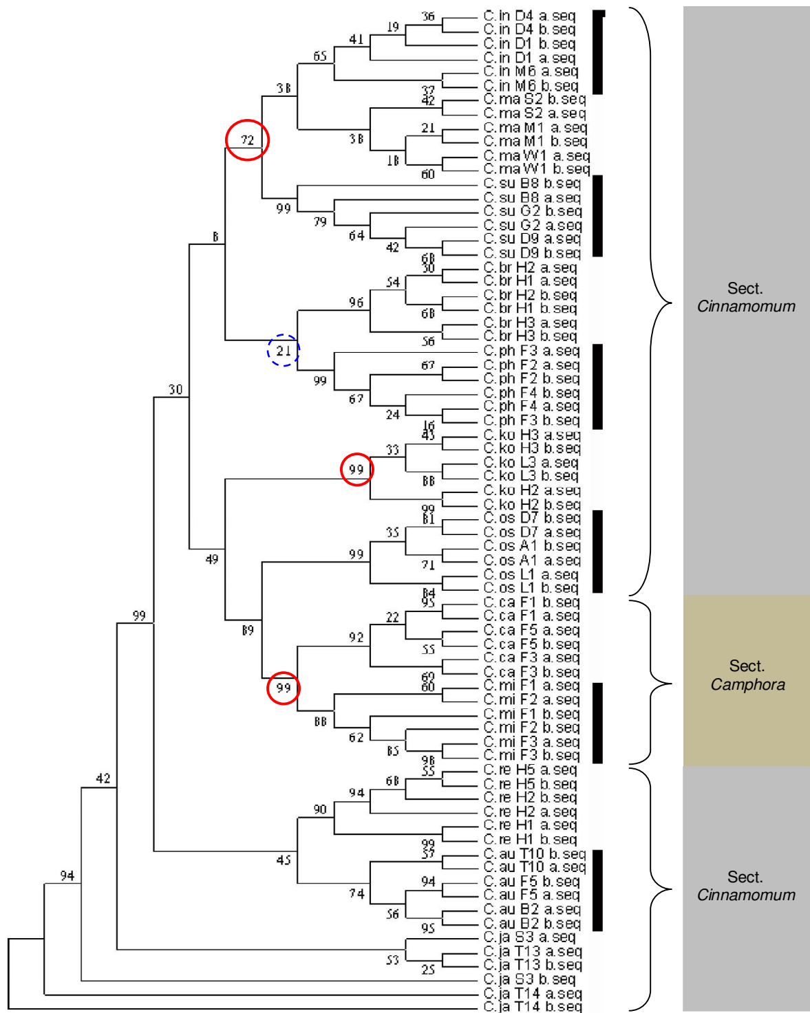
Figure 6. MP consensus tree constructed based on ITS sequences.
