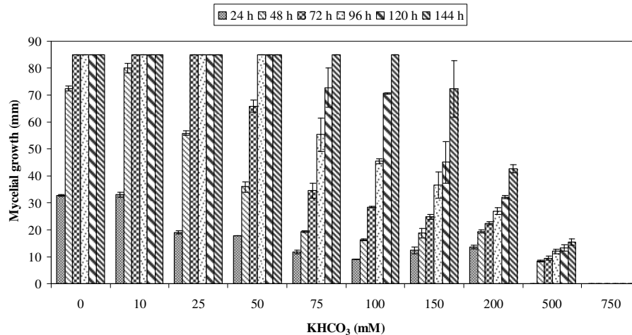
Figure 1. Time relevant in vitro mycelial growth of Rhizoctonia solani AG 4 HG-I exposed to potassium bicarbonate ( \text{KHCO}_3 ). Vertical lines represent standard errors of the means.
