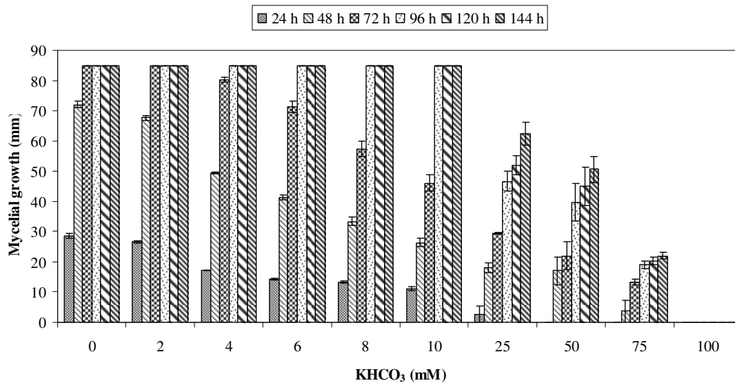
Figure 4. Time relevant in vitro mycelial growth of Trichoderma sp. exposed to different concentrations of potassium bicarbonate (KHCO 3 ). Vertical lines represent standard errors of the means.
