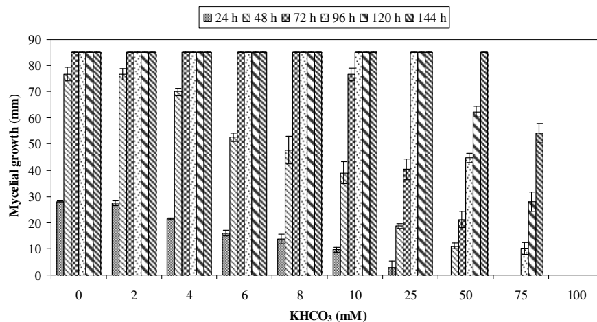
Figure 2. Time relevant in vitro mycelial growth of Sclerotinia sclerotiorum exposed to potassium bicarbonate ( \text{KHCO}_3 ). Vertical lines represent standard errors of the means.
