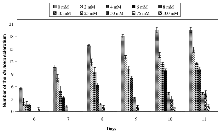
Figure 6. Effects of increasing concentrations of potassium bicarbonate ( \text{KHCO}_3 ) on de novo sclerotium formation by Sclerotinia sclerotiorum after the fifth days of sclerotium germination. Vertical lines represent standard errors of the means.
