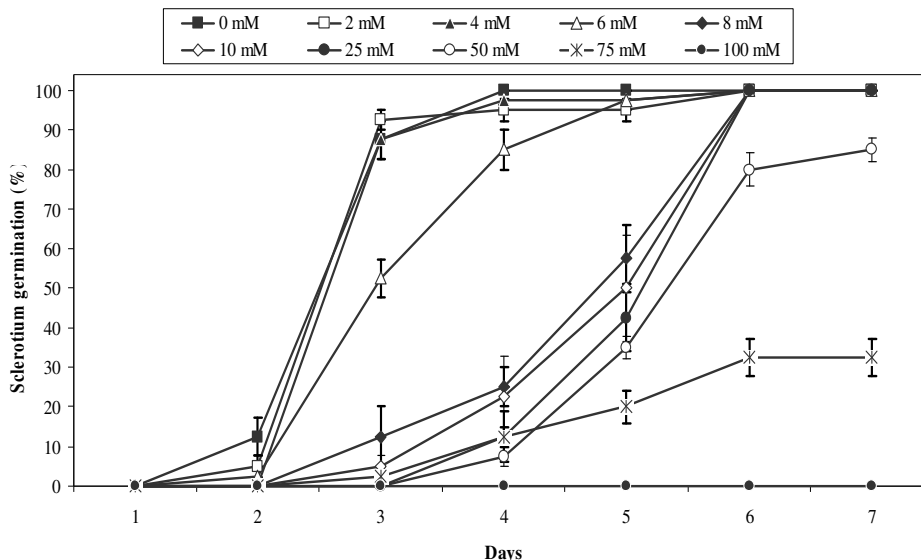
Figure 5. Germination (%) of the sclerotia of Sclerotinia sclerotiorum exposed to different concentrations of potassium bicarbonate ( \text{KHCO}_3 ) after 168 hours in vitro . Vertical lines represent standard errors of the means.
