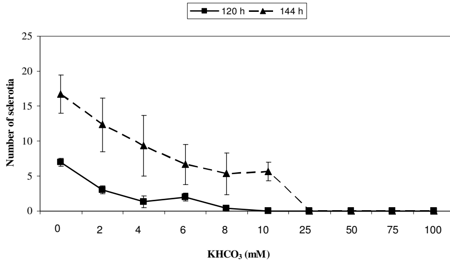
Figure 3. Effect of potassium bicarbonate (KHCO 3 ) concentrations on the number of sclerotia of Sclerotinia sclerotiorum , after 120 and 144 h. Vertical lines represent standard errors of the means.
