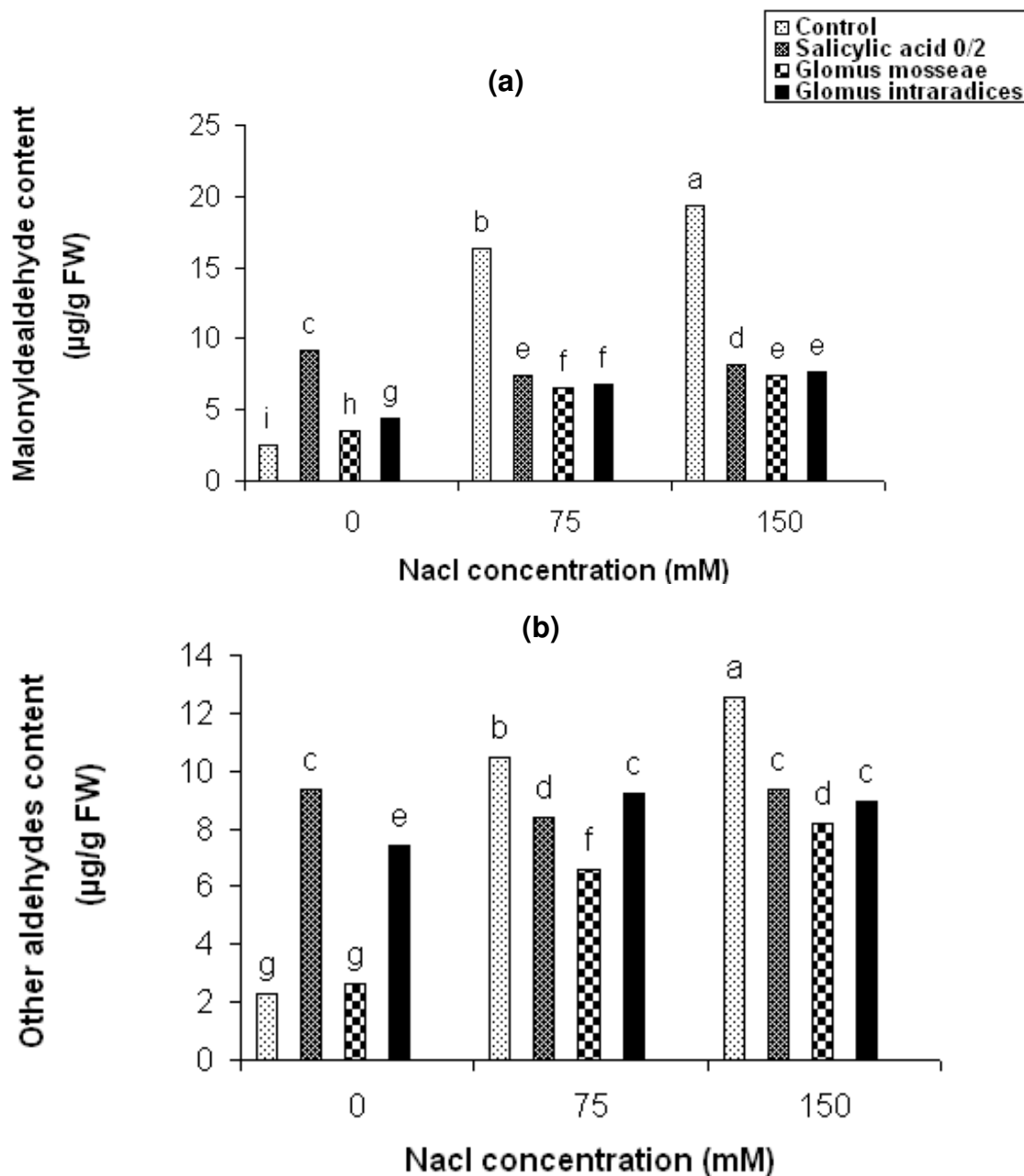
Figure 2. Interactive effect of mycorrhizal fungus, salicylic acid and salinity on the content of malondialdehyde (a) and other aldehydes (b).
