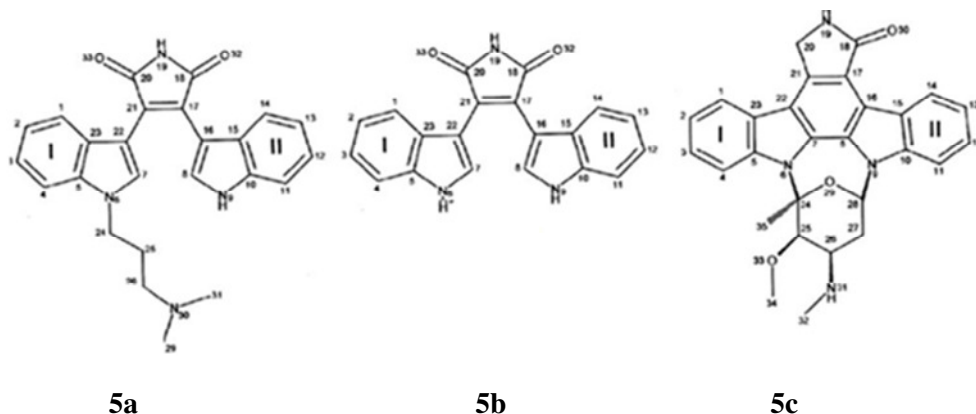
Figure 5. Structural analysis of the three inhibitors used for docking within the model protein PKC \beta -I. 5a, BIM-1 (2-methyl-1H-indol-3-yl); 5b, balanol; 5c, staurosporine. The two indole rings present in 5a, 5b and 5c are designated by roman numerals I and II.
