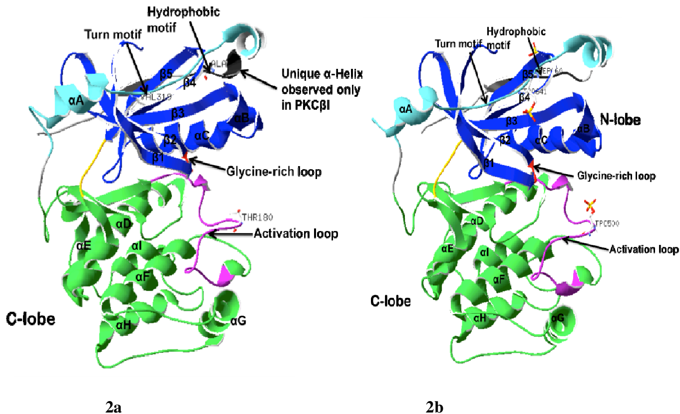
Figure 2. Analysis of structure. 2a; Catalytic domain of PKC \beta -I. The N-lobe is given in dark blue and C-lobe in green. The glycine rich loop is highlighted in red, activation loop in pink and phosphorylated residues are given in stick representation. A unique \alpha -helix is shown in black. 2b; Catalytic domain of PKC \beta -II. The N-lobe is given in dark blue and C-lobe in green. The glycine rich loop is highlighted in red, activation loop in pink and phosphorylated residues are given in stick representation.
