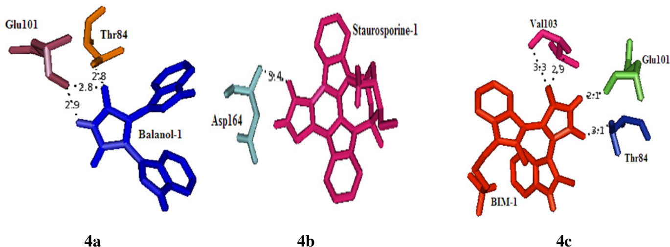
Figure 4. 4a; Four polar interactions between BIM-1 and PKC \beta I including Glu 101(H-O=2.1 Å), Val 103 (O-N=2.9 Å, O-O=3.3 Å) and Thr 84 (O-O=3.1 Å); 4b, three polar interactions between balanol-1 including two with Glu 102 (H-O=2.9 Å, O-O=2.8 Å) and one with Thr 84(O-O=2.8 Å); 4c, only one polar interaction between staurosporine-1 and PKC \beta I that was with Asp 164 (O-N=3.4 Å).
