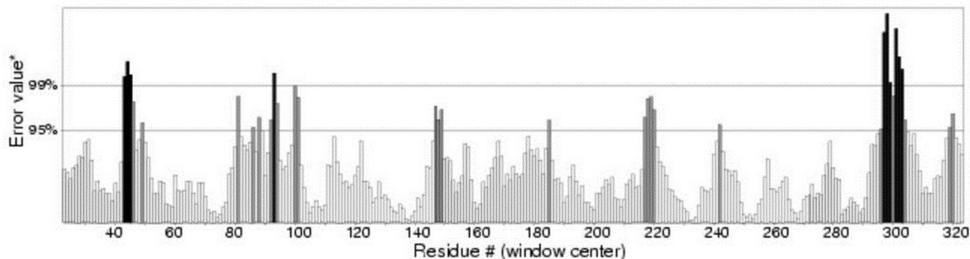
Figure 1. Graphical representation by ERRAT. Here in this graph, on the error axis two lines are drawn to indicate the confidence with which it is possible to reject regions that exceed the error value. Overall quality factor was 88.923, for which the calculated error value falls below 95% rejection limit.
