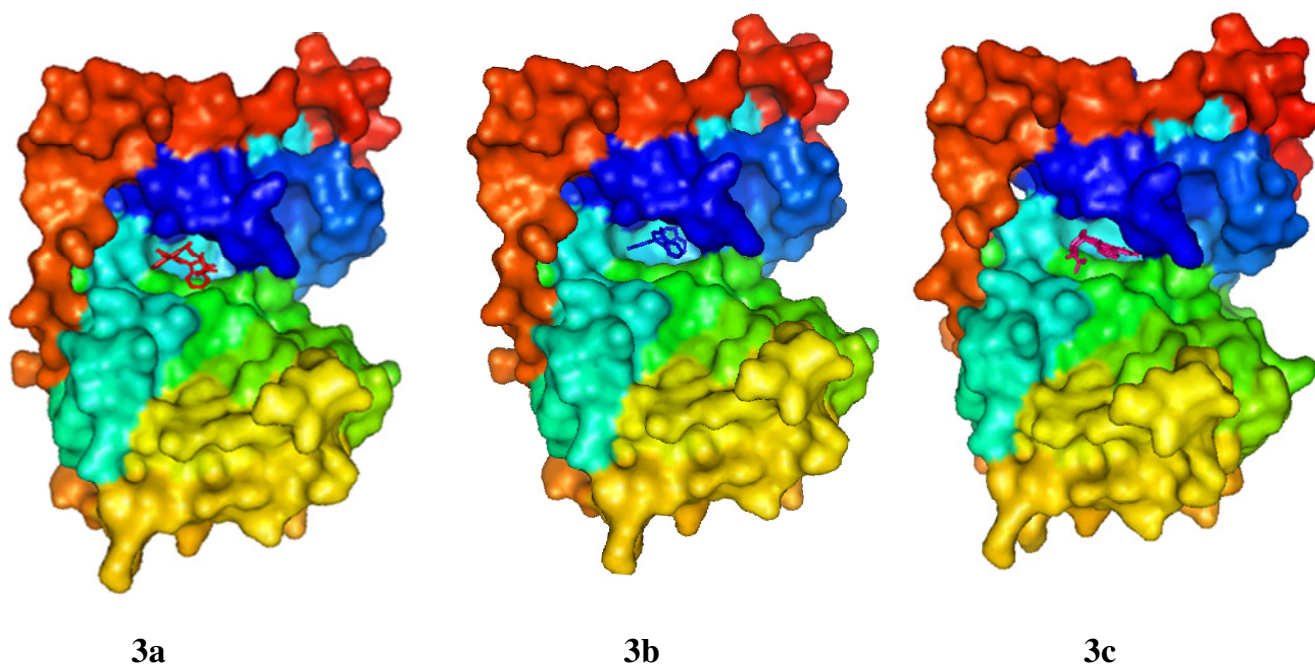
Figure 3. Analysis of docking. 3a, Docking of 2-methyl-1H-indol-3-yl-BIM-1 into the cleft of PKC \beta -I; 3b, docking of balanol-1 into the cleft of PKC \beta -I; 3c, docking of staurosporine-1 into the cleft of PKC \beta -I.
