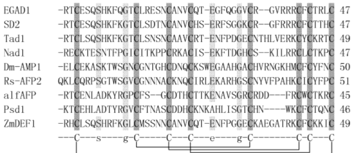
Figure 2. Amino acid sequence alignment of mature plant defensins from several plants. Comparison of the deduced mature ZmDEF1 amino acid sequence with those of other plant defensins. Conserved residues are presented in black boxes, partially conserved residues in gray boxes, while the defensin consensus sequence is shown below the alignment. The disulfide bond connectivities are shown below the consensus sequence by connecting lines. The sequences were aligned using the CLUSTALW2 online ( http://www.ebi.ac.uk/Tools/msa/clustalw2/ ).
