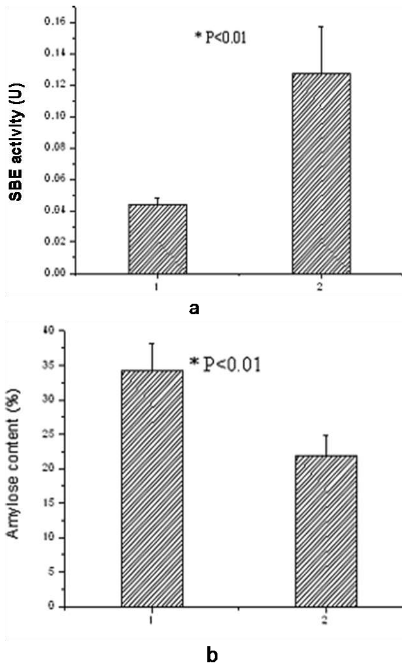
Figure 7. SBE activity and amylose percent contents in kernels and seeds of T_1 transgenic plants. SBE activity assay was performed in kernels according to Li et al. (1997) with slight modification. The starch contents were determined using a dual wavelength method as reference (Hovenkamp-Hermelink et al., 1988). Each treatment was repeated three times. Total starch was the sum of amylopectin and amylose. (a) SBE activity; (b) amylose percent content; 1, transgenic plant (H99-1); 2, non-transgenic plant.
