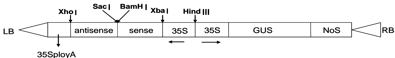
Figure 1. The structure map of T-DNA region in RNAi vector pRSBE2a. PCR products of sbe2a were excised with XbaI + BamHI and SacI + XhoI producing specific 562 bp fragments and ligated to modified pCambia1301 vector as the sense and antisense segments, respectively.
