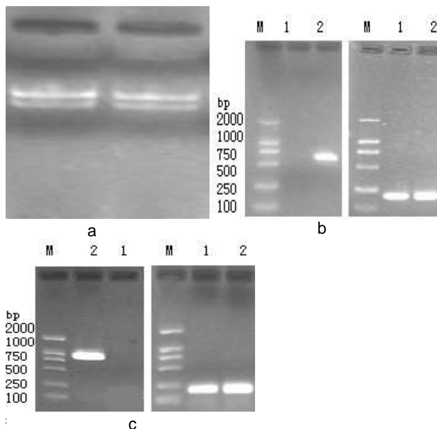
Figure 6. RT-PCR analysis of transgenic plants. The endogenous SBE mRNA content was analyzed in transgenic plants. (a) Total RNA extracts from maize kernels; (b) reaction for 28 cycles; (c) reaction for 30 cycles; M, DNA marker DL-2000; 1, transgenic plant (H99-1); 2, non-transgenic plant; Sbe2a segment, 562 bp; EF-1 a , 213 bp.
