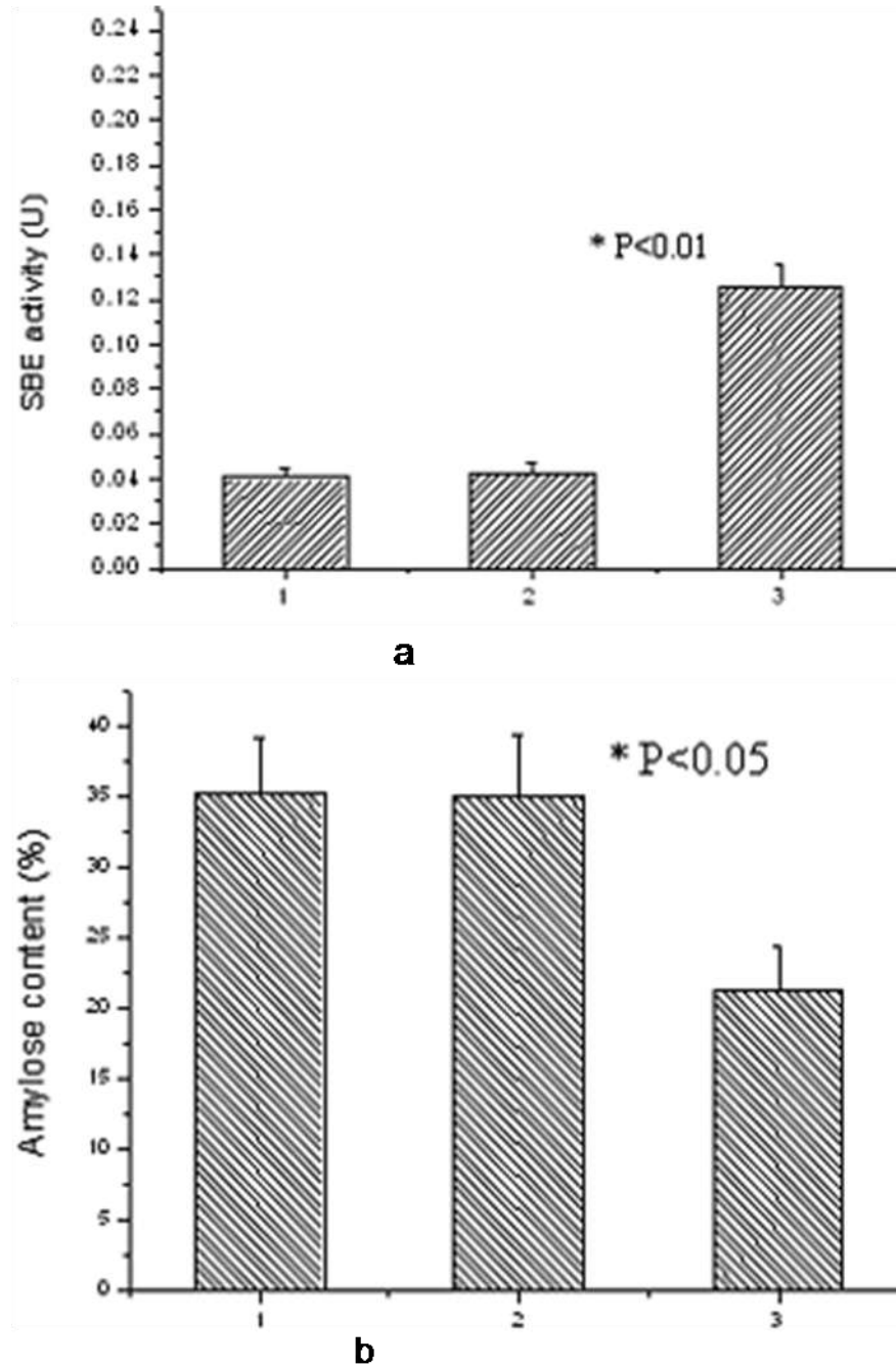
Figure 8. SBE activity and amylose percent contents in seeds of T_2 transgenic plants. SBE activity assay was performed in kernels according to Li et al. (1997) with slight modification. The starch contents were determined using a dual wavelength method as reference (Hovenkamp-Hermelink et al., 1988). Each treatment was repeated three times. Total starch was the sum of amylopectin and amylose. (a) SBE activity; (b) amylose content; 1, 2, transgenic plants (H99-1-1, H99-1-2); 3, non-transgenic plant.
