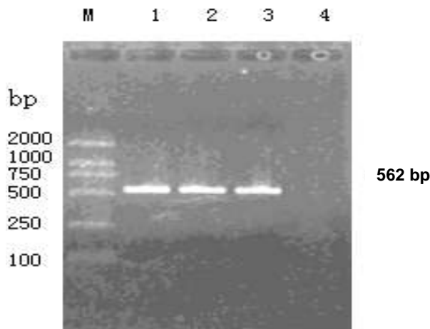
Figure 2. Isolation of starch branching enzyme sbe2a gene. The 562 bp sbe2a fragment was obtained from RT-PCR products of maize W1. M, DNA Marker DL-2000; 1-3, PCR products; 4, negative control.
