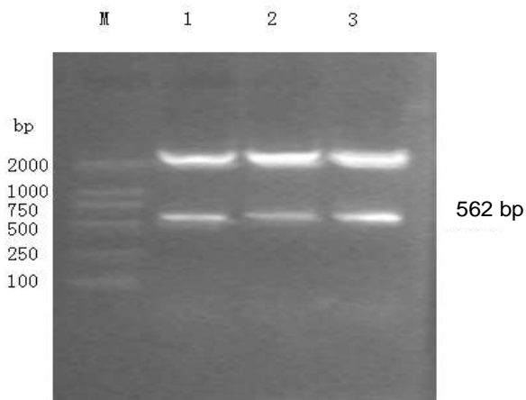
Figure 3. Restriction enzyme analysis of the recombinant clone. The plasmid DNA of positive colonies was extracted and digested by Sac I + Xho I. Then DNA electrophoresis was performed. M, DNA marker DL-2000; 1,2,3, pMD18-T-SBEIIa/ Sac I + Xho I.
