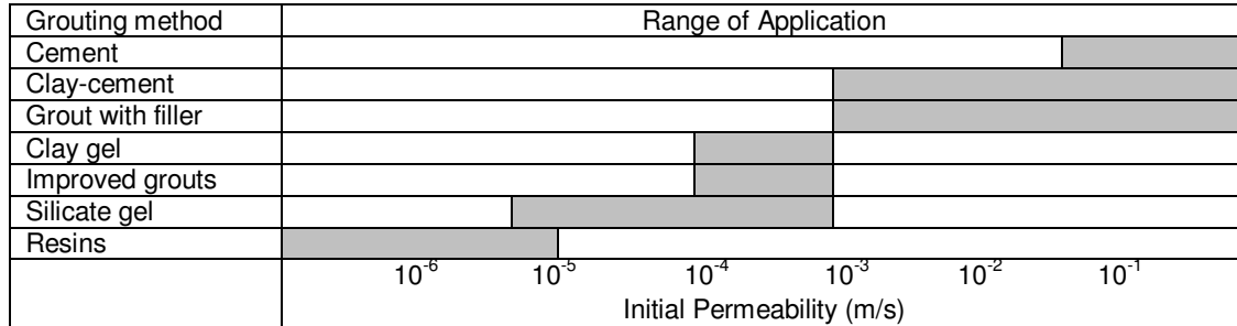
Figure 1. Applications of grouts for granular soils.
