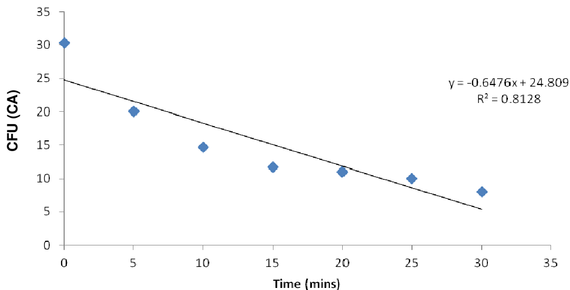
Figure 1. Zero-order kinetics plot.
