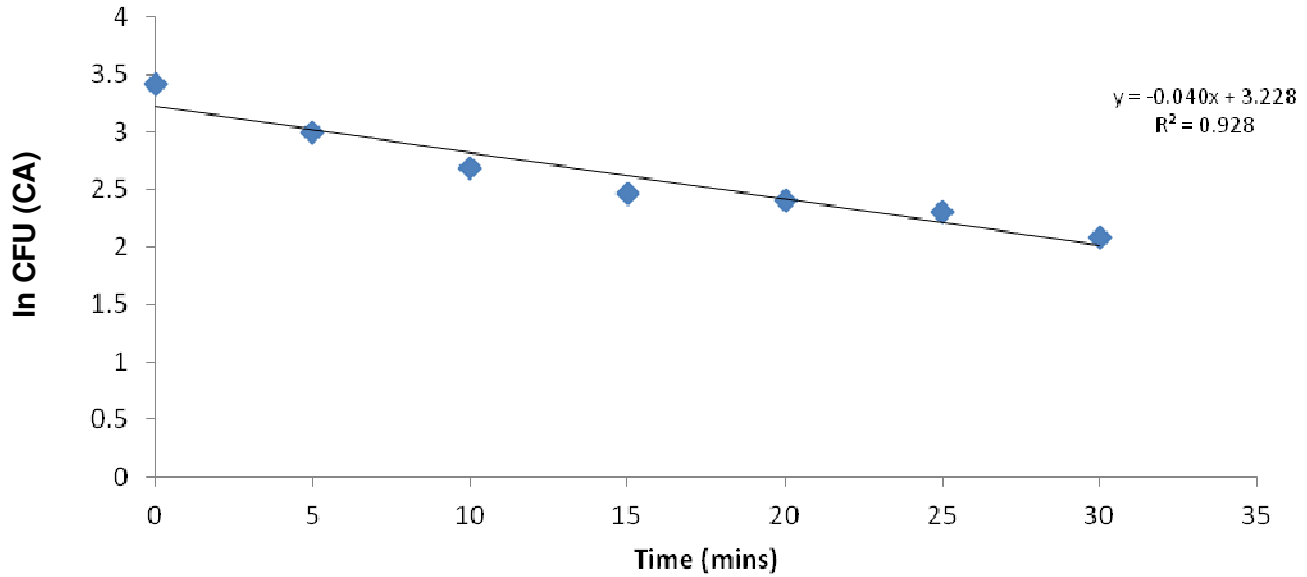
Figure 2. First-order kinetics plot.
