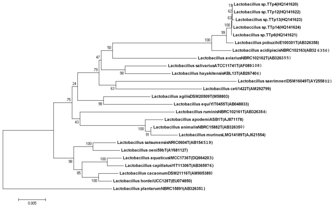
Figure 1. Neighbor-joining phylogenetic tree based on 16S rRNA gene sequence comparisons showing the position of strain Lactobacillus sp. (TTP4, TTP6, TTP12, TTP13 and TTP14) and related Lactobacilli (bootstrap values are indicated at branch points based on 1000 replications). The sequence of Lactobacillus plantarum NBRC 15891T was used as an outgroup. GenBank accession numbers are given in parentheses
