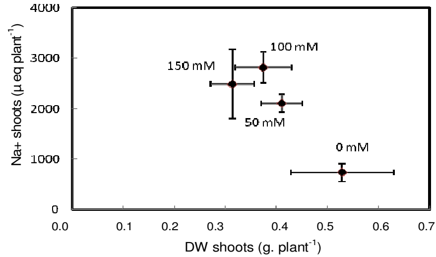
Figure 3. Correlation between Na content and the shoots biomass of Cymbopogon schoenanthus cultivated under salt stress. The duration of the treatment was 30 days and the plants were cultivated in the presence of NaCl (from 0 to 150 mM).
