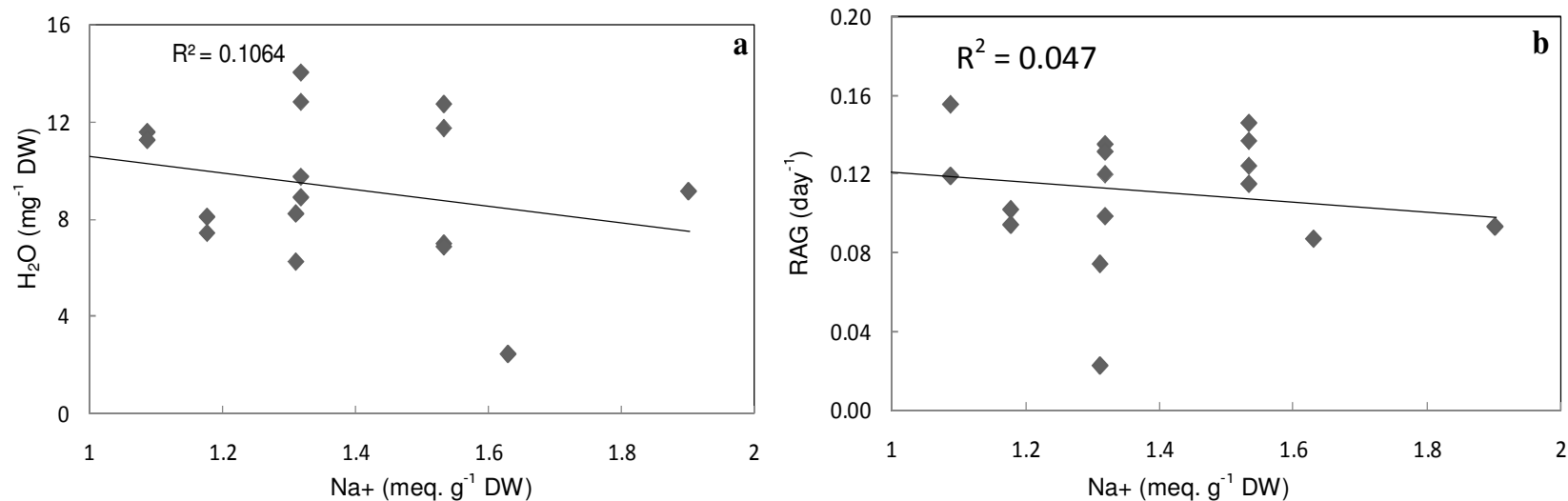
Figure 1. Correlation between water content and the Na content (a), and the RAG and the Na content (b) of the shoots of Cymbopogon schoenanthus cultivated under salt stress. The duration of the treatment was 30 days.
