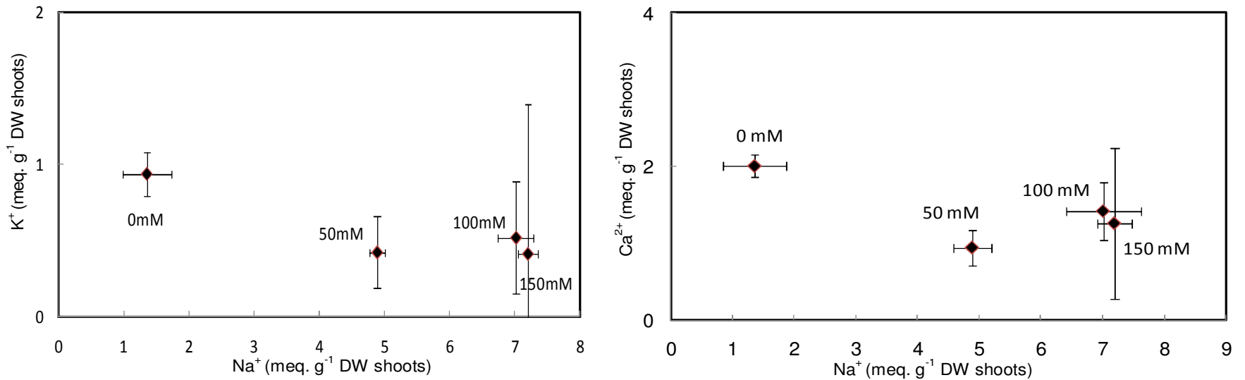
Figure 4. Absorption selectivity of K^+/Na^+ and Ca^{2+}/Na^+ in the shoots of Cymbopogon schoenanthus according to different NaCl concentrations.
