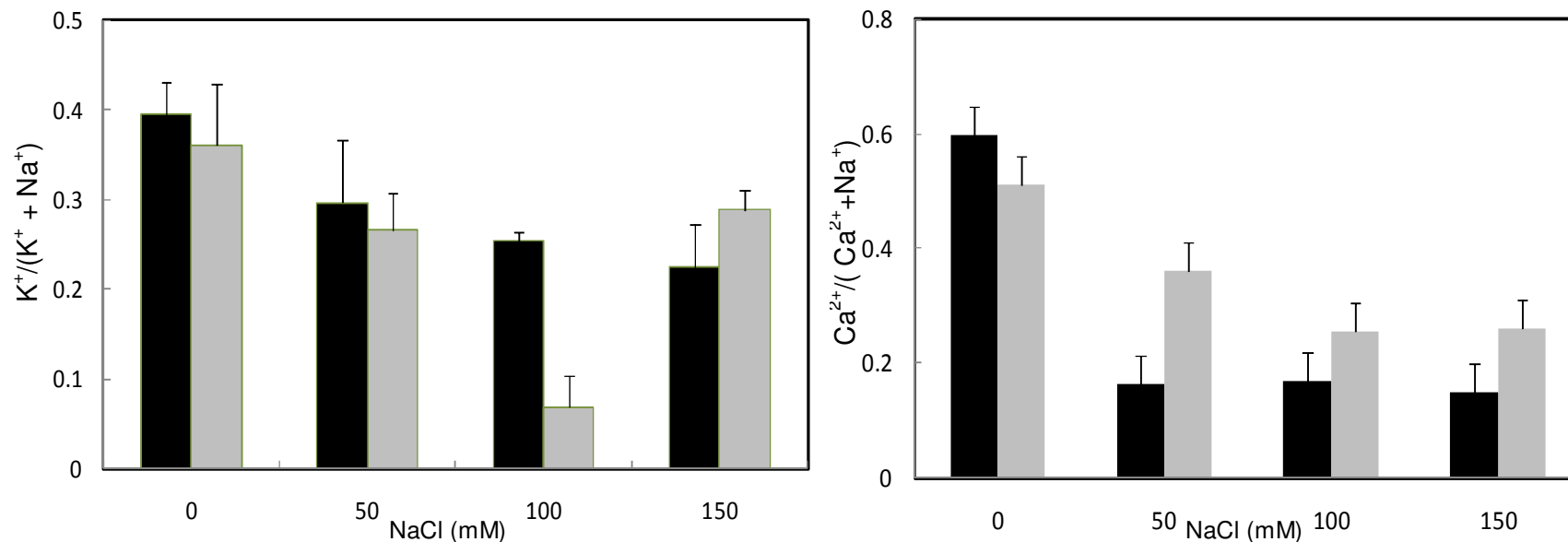
Figure 2. Ratios of K^+/(K^+ + Na^+) and Ca^{2+}/(Ca^{2+} + Na^+) in the roots and shoots of Cymbopogon schoenanthus according to different concentrations of NaCl. Treatment duration was 30 days.
