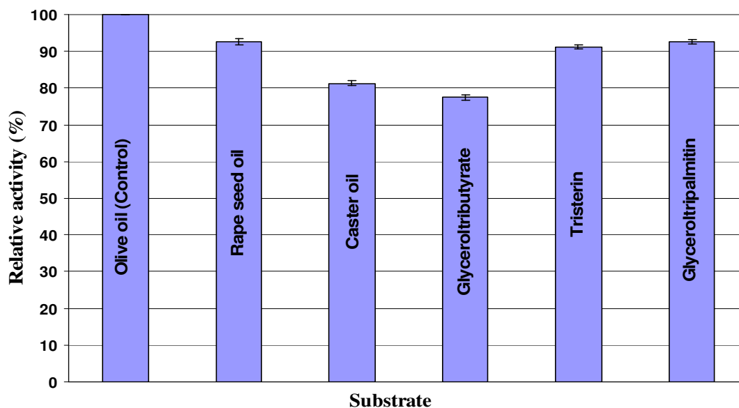
Figure 3. Effect of substrate specificity on lipase activity produced by M. geophillus
