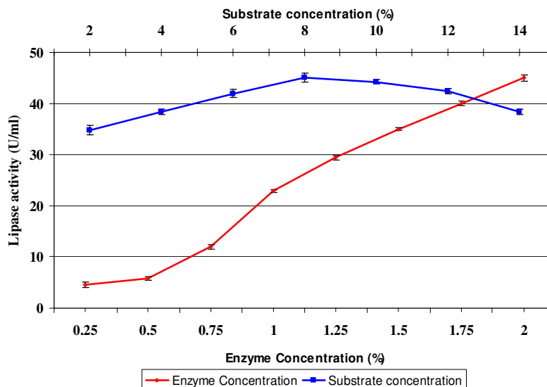
Figure 4. Effect of substrate (olive oil) and enzyme concentrations on lipase activity produced by M. geophillus . The enzyme was measured at pH 6.5, and 35°C.
