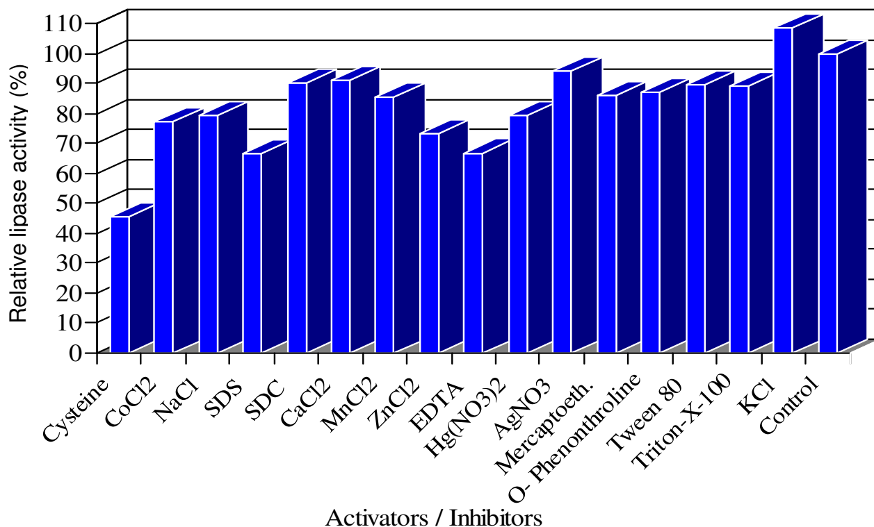
Figure 8. Effect of various activators and inhibitors on lipase activity produced by M. geophilus .
