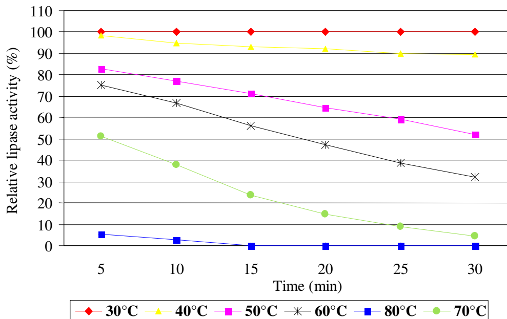
Figure 7. Effect of thermal stability at various time periods on lipase activity produced by M. geophilus .
