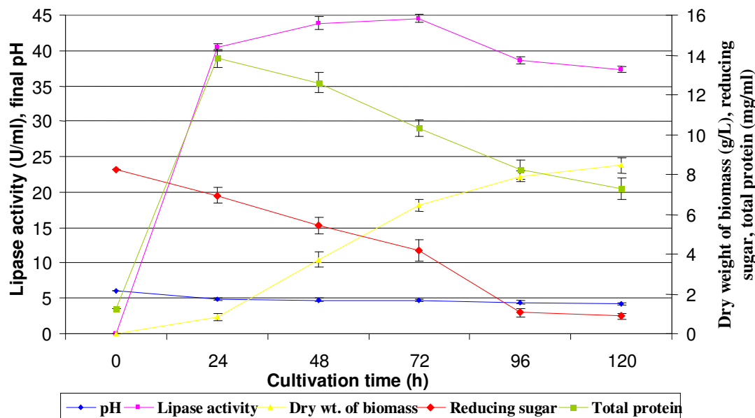
Figure 1. Lipase production by M. geophillus grown on 5% molasses at 30 \pm 2^\circ\text{C}
