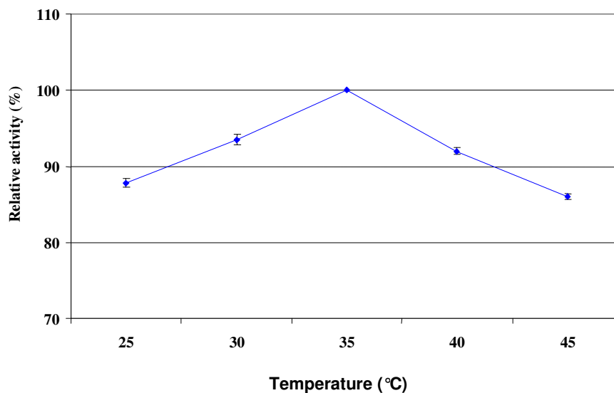
Figure 6. Effect of temperature on lipase activity produced by M. geophillus . The enzyme was measured at pH 6.5.
