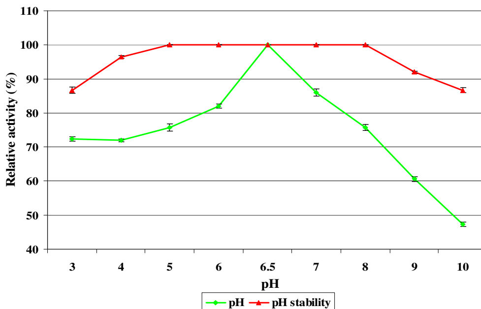
Figure 5. Effect of pH and pH stability on lipase activity produced by M. geophillus .
