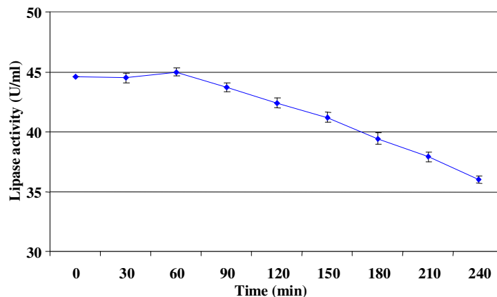
Figure 2. Effect of time on lipase activity produced by M. geophillus . The enzyme was measured at pH 6.5, and 37°C.
