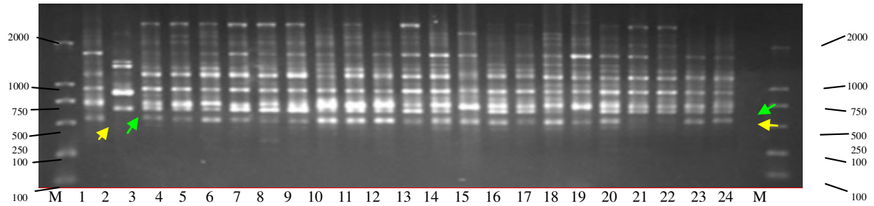
Figure 3. Results of hybrids identifications with RAPD molecular marker in “Yacheng 89/9× Erianthus fulvus ” F 1 (Primer OPN-11). Lane M, DNA marker; Lane 1, Yacheng89/9; Lane 2, Erianthus fulvus ; Lane 3-23, different hybrid F 1 accessions; Lane 24, control; yellow arrows in the figure indicated maternal-specific band; green arrows in the figure indicate paternal-specific band.
