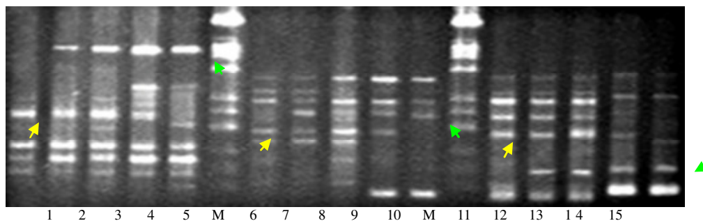
Figure 1. RAPD products obtained from sugarcane hybrids and its parents with three primers. Lane M, DNA marker ( \lambda DNA/ EcoR \square + Hind \square ); Line 1-5, accessions amplified by OPC-19 (Lane 1, Yacheng89/9; Lane 5, Erianthus fulvus ; Lane 2-4, different hybrid F 1 accessions; yellow arrows in line 1 indicated maternal-specific band OPC-19 3500 ); Line 6-10, accessions amplified by OPE-02 (Lane 6, Yacheng89/9; Lane 10, Erianthus fulvus ; Lane 7-9, different hybrid F 1 accessions; yellow arrows in line6 indicated maternal-specific band OPE-02 900 ; green arrows in line10 indicate paternal-specific band OPE-02 1350 ); Line 11-15, accessions amplified by OPF-04 (Lane 11, Yacheng89/9; Lane 15, Erianthus fulvus ; Lane 12-14, different hybrid F 1 accessions; yellow arrows in line 11 indicated maternal-specific band OPF-04 900 ; green arrows in line 15 indicate paternal-specific band OPF-04 550 ).
