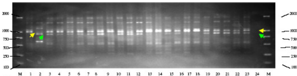
Figure 2. Results of hybrids identifications with RAPD molecular marker in "Yacheng 89/9× Erianthus fulvus " F 1 (Primer OPN-11). Lane M, DNA marker; Lane 1, Yacheng89/9; Lane 2, E. fulvus ; Lane 3-23, different hybrid F 1 accessions; Lane 24, control; yellow arrows in the figure indicated paternal-specific band; green arrows in the figure indicate maternal-specific band.
