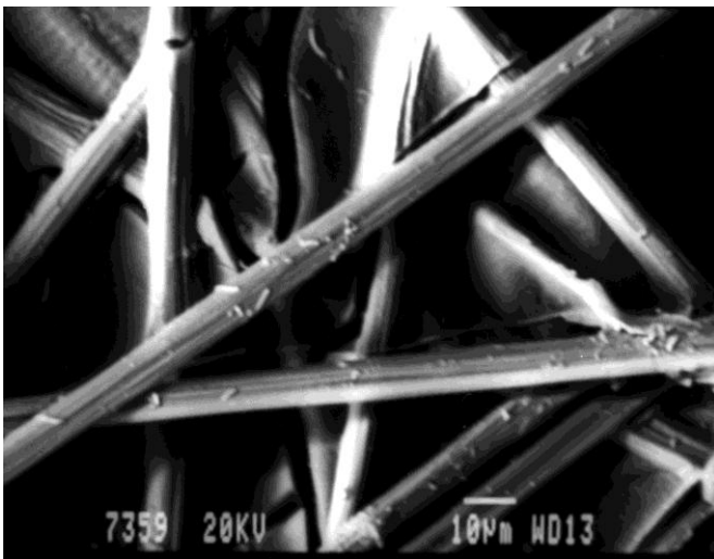
Figure 3. A scanning electron micrograph of a sparsely colonised anode electrode.
