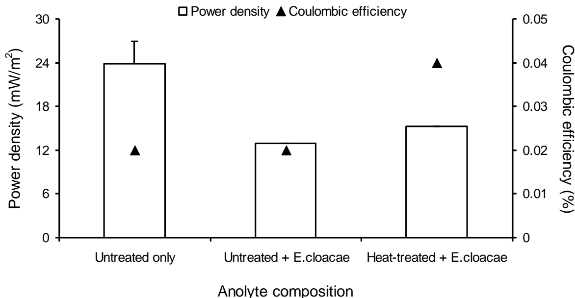
Figure 1. Maximum power densities and respective coulombic efficiencies from different MFC setups fed with paper mill effluent.
