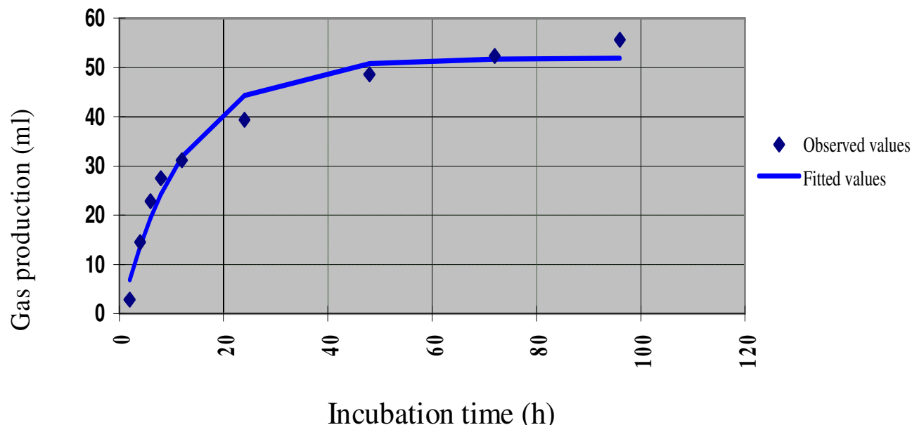
Figure 1. In vitro gas production volume of tomato pomace at different incubation time.
