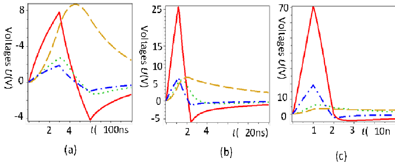
FIGURE 3. Induced voltages U(V) vs. elapsed time t from (a)300ns, 26kV/cm PEF; (b)60ns, 60kV/cm PEF; (c)10ns,150kV/cm PEF. — nucleus (NP), — Plasma membrane (PM), —•— cytoplasm(CP),•••Nuclear envelope(NE)
