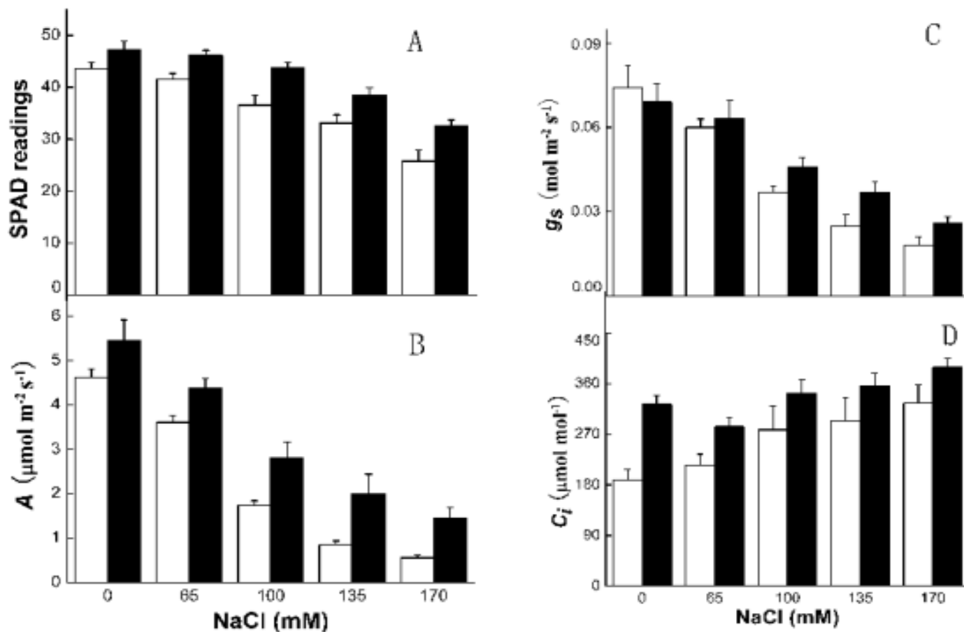
Figure 3. Effects of increasing NaCl concentration on chlorophyll content (A), photosynthetic rate (B), stomatal conductance (C) and intercellular \text{CO}_2 concentration (D) of two Elytrigia species, E. trichophora (open columns) and E. intermedia (closed columns), exposed to five NaCl treatments over 21 days. Vertical bars represent mean \pm S.E. ( n = 3 ).
