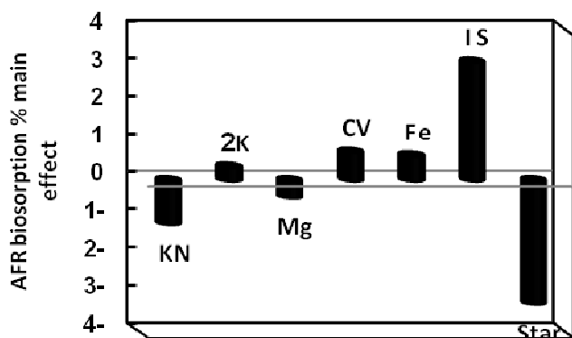
Figure 2. The main effects of different factors affecting acid fast red biosorption (%) by S. globosus under static conditions.
