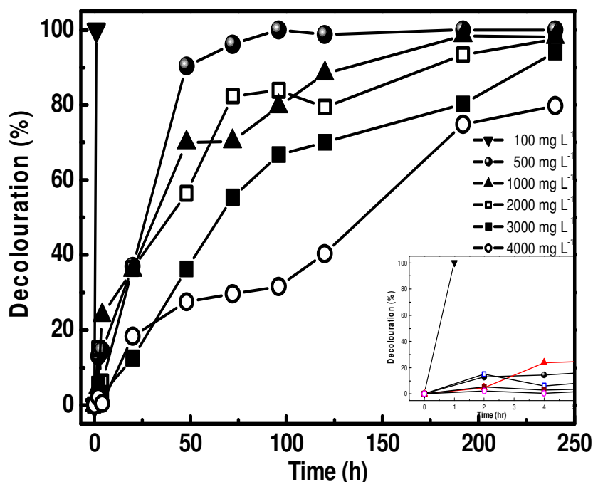
Figure 1. Effect of IC concentration reaction conditions: 6 g lyophilized mycelia /L of IC solution, room temperature, 17.8 \times g in non-buffered media. Concentration IC: ( \blacktriangledown ), 100 \text{ mg l}^{-1} , ( \bullet ), 500 \text{ mg l}^{-1} , ( \blacktriangle ), 1\ 000 \text{ mg l}^{-1} , ( \square ), 2\ 000 \text{ mg l}^{-1} , ( \blacksquare ), 3\ 000 \text{ mg l}^{-1} , ( \circ ) 4\ 000 \text{ mg l}^{-1}
