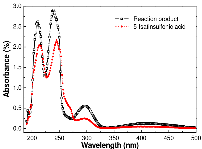
Figure 3. UV-VIS spectra of 5-isatinsulfonic acid and product reaction. Reaction condition: IC 4\ 000 \text{ mg L}^{-1} with lyophilized mycelia, at room temperature, in a non-buffered media; concentration of mycelium/colorant 14 \text{ g L}^{-1} and 17.8 \times g ; (●) —, 5-isatinsulfonic acid; (□), reaction product.
