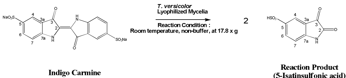
Figure 5. Chemical reaction of Indigo carmine with T. versicolor lyophilized mycelia. Reaction condition: room temperature and a non-buffer at 17.8 \times g .
