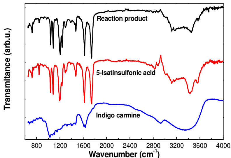
Figure 4. FT- IR spectra comparison of 5-isatinsulfonic acid and the reaction product in the frequency region of 800 to 4 000 \text{cm}^{-1} . —, 5-isatinsulfonic acid; —, reaction product; —, indigo carmine.
