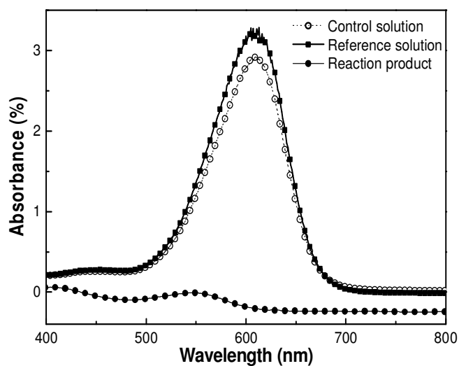
Figure 2. UV-VIS spectra of 100 \text{ mg l}^{-1} IC with lyophilized mycelia of T. versicolor after 1 h of reaction, with 6 \text{ g mycelia/L} , at room temperature and 17.8 \times g in non-buffered medium. (■), reference solution (IC); (○), control solution; (●), reaction product.
