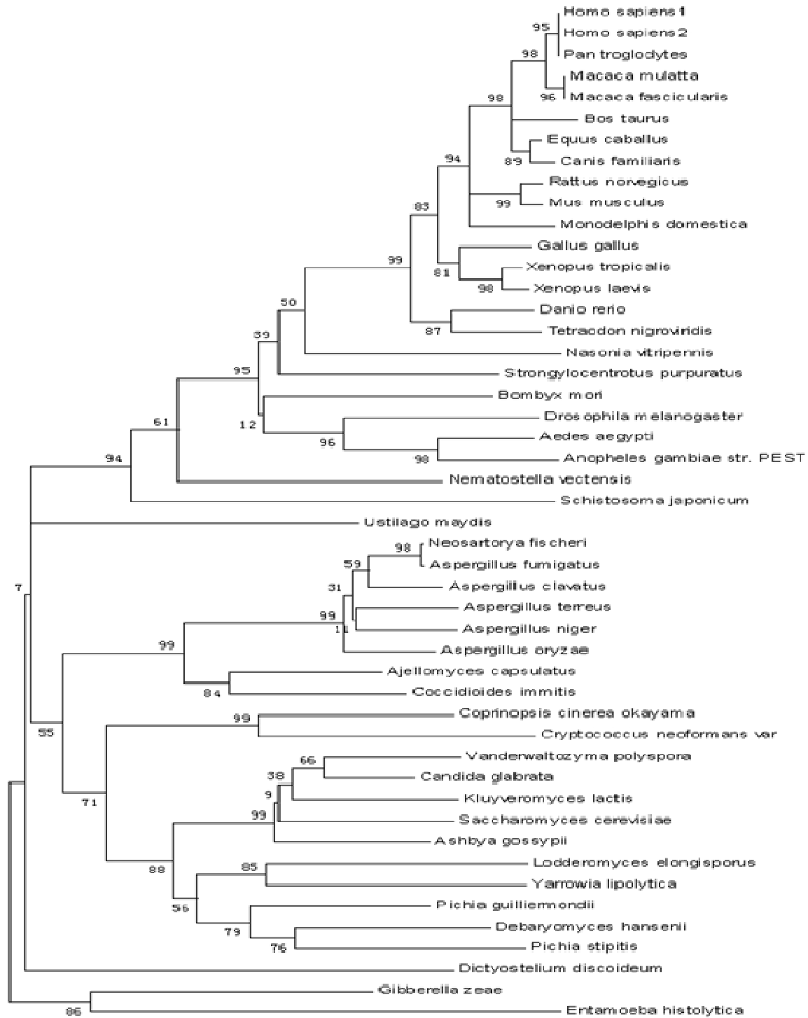
Figure 3. Phylogenetic tree of BmLOC77850.
