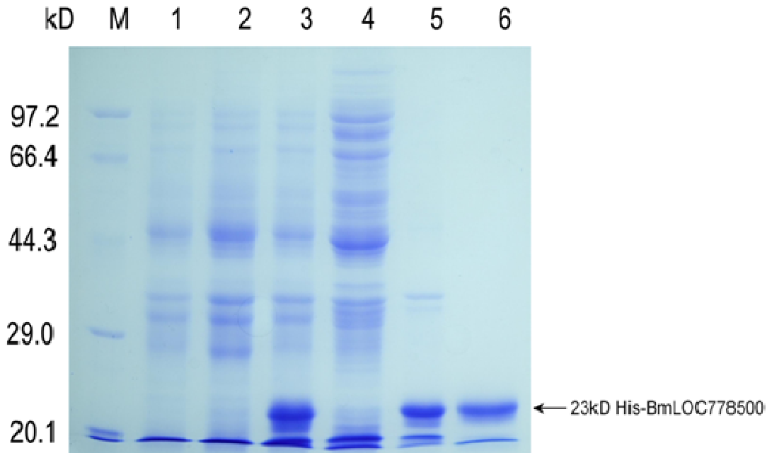
Figure 4. Expression and purification of the fusion protein His-BmLOC778500. The fusion protein His-BmLOC778500 purified by Ni-NTA were analyzed by SDS-PAGE and visualized by Coomassie brilliant blue R-250 staining. M, Molecular weight markers with the masses shown, in kilodalton, to the left; 1, negative control; 2, the total protein of lysate from uninduced BL21(DE3)-pET-28a- BmLOC778500 ; 3, the total protein of lysate from BL21(DE3)-pET-28a- BmLOC778500 after inducing with IPTG for 5 h; 4, the lysate precipitation from BL21(DE3)-pET-28a- BmLOC778500 after inducing with IPTG for 5 h; 5, the lysate supernatant from BL21(DE3)-pET-28a- BmLOC778500 after inducing with IPTG for 5 h; 6, the purified proteins His-BmLOC778500.
