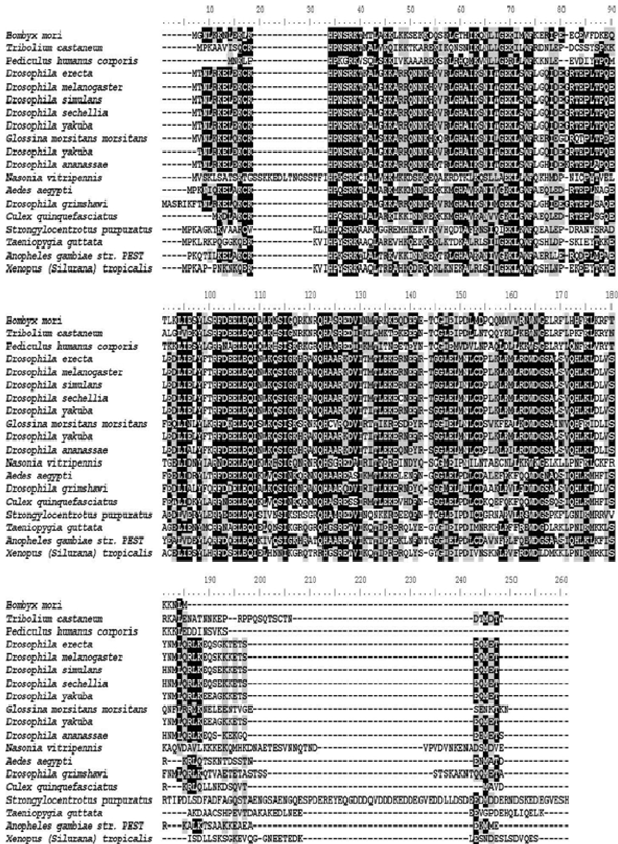
Figure 2. Multiple sequence alignment of BmLOC77850. Black-shaded amino acids indicate identical residues; gray-shaded amino acids indicate similar residues.
