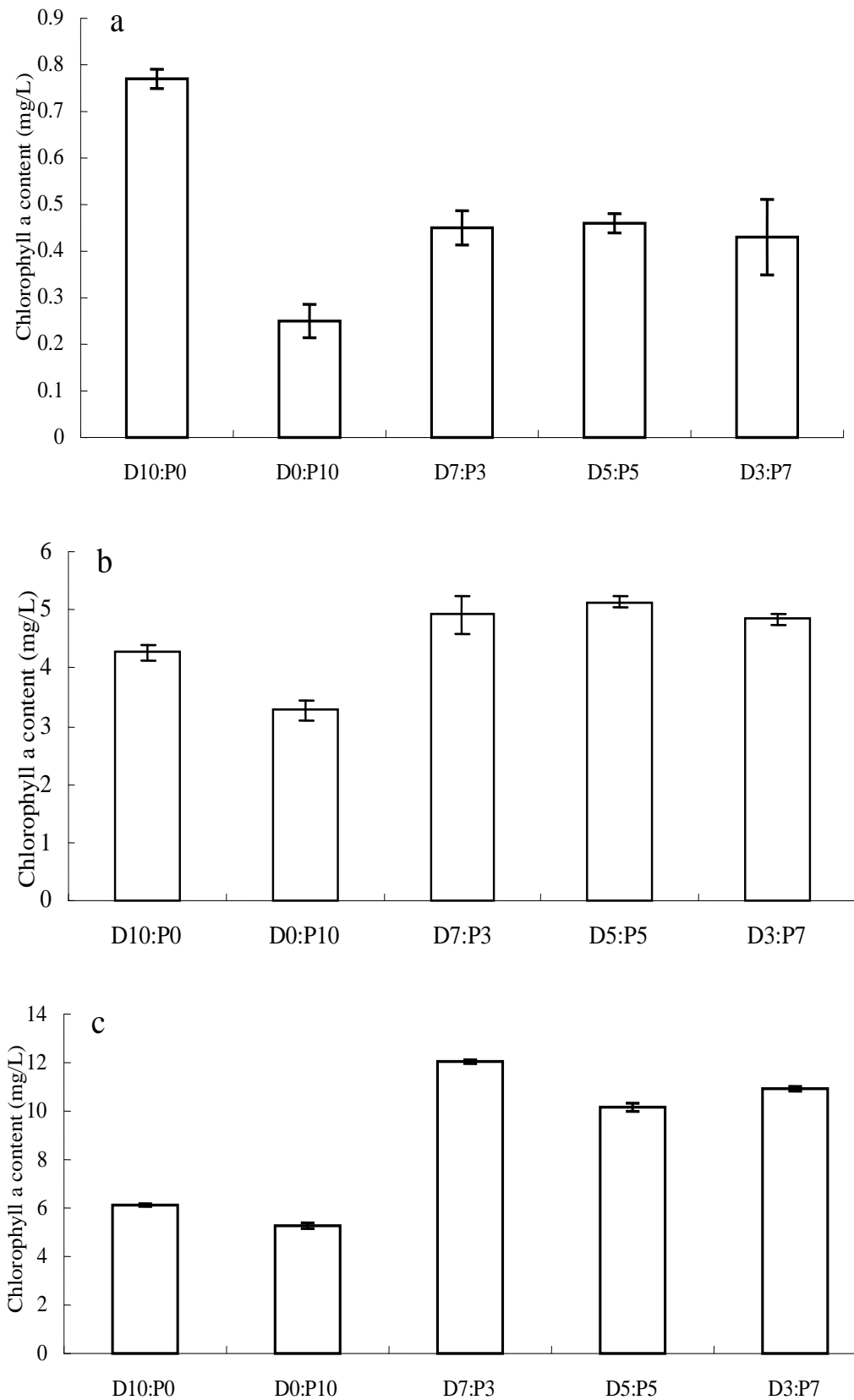
Figure 4. Microalgal chlorophyll a content of D. salina (D) and P. tricornutum (P) under different
