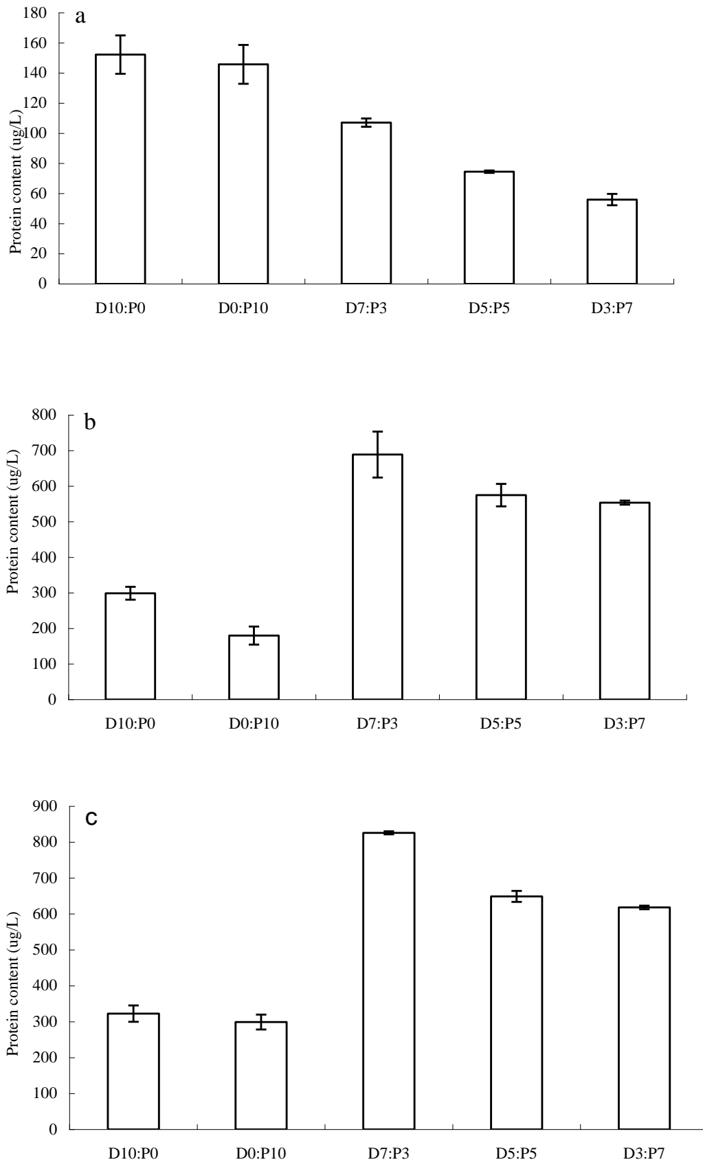
Figure 5. Microalgal protein content of D. salina (D) and P. tricornutum (P) under different
