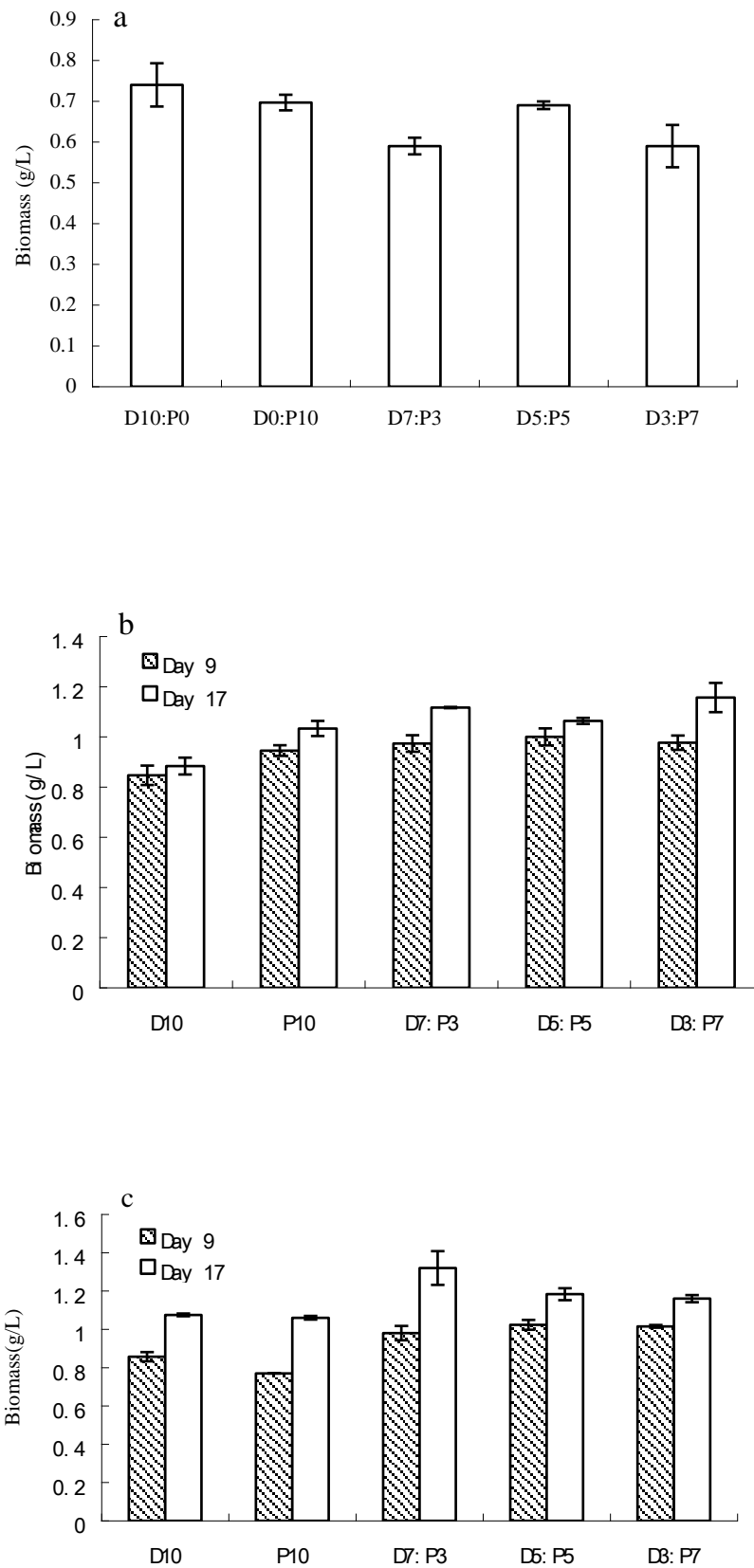
Figure 3. Microalgal biomass of D. salina (D) and P. tricornutum (P) at different sampling time under various inoculation density and nitrogen
