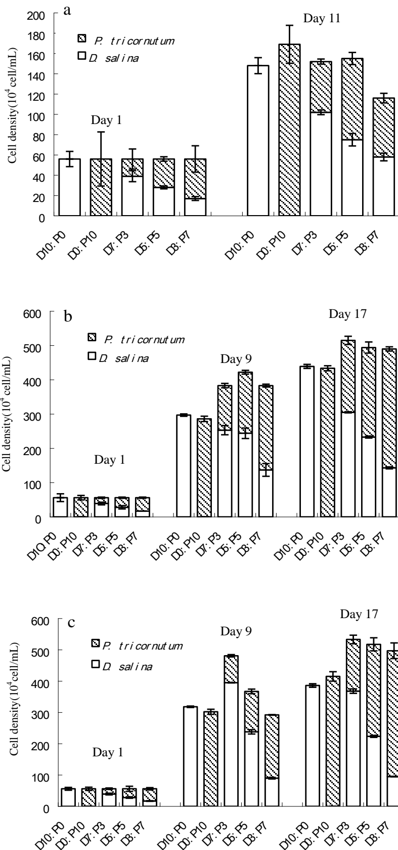
Figure 2. Microalgal cell density of D. salina (D) and P. tricornutum (P) at different sampling time under various inoculation density and nitrogen
