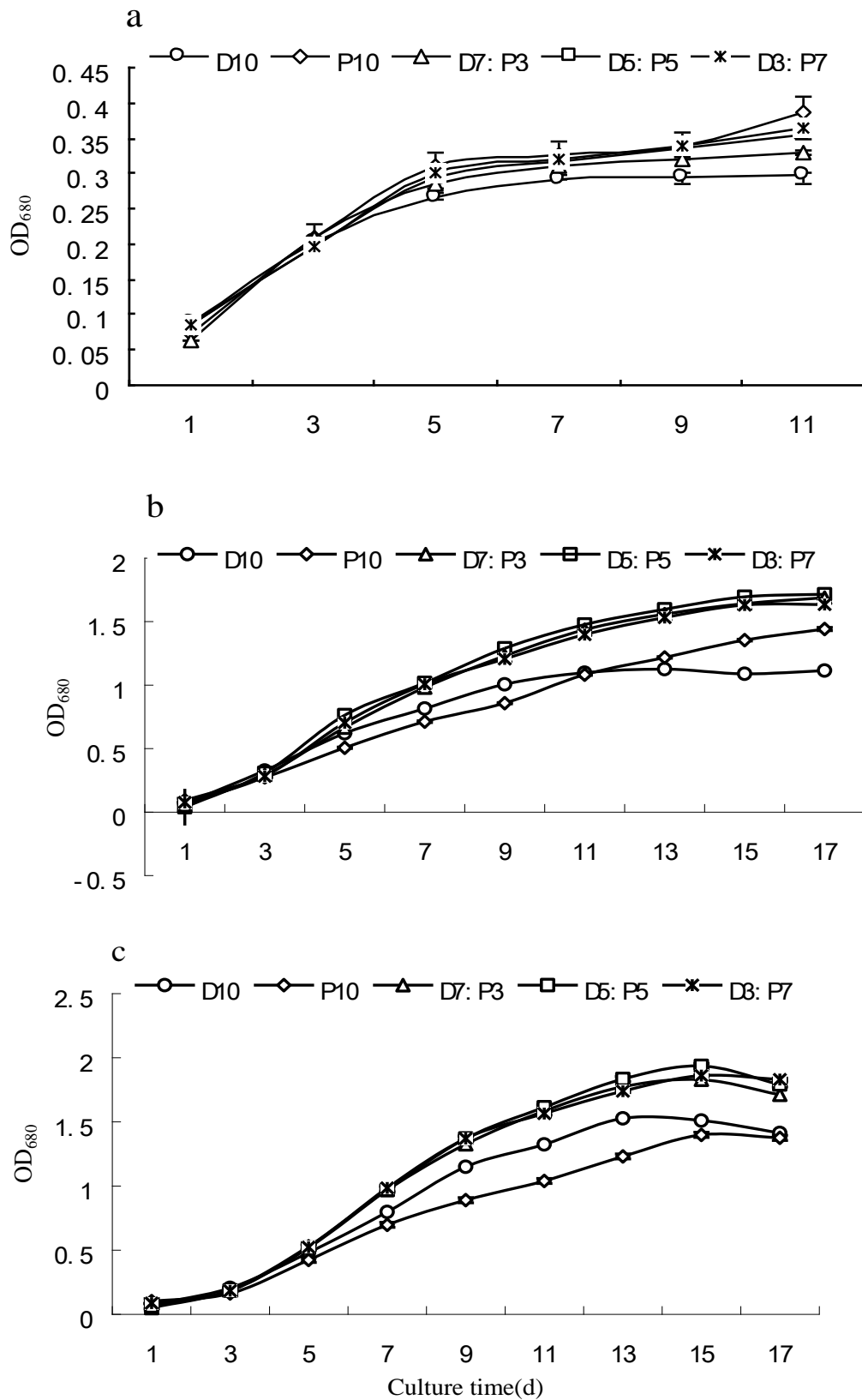
Figure 1. Value of OD 680 of D. salina (D) and P. tricornutum (P) under different inoculation density and nitrogen concentration. A: 1.4 mg/l; B: 14 mg/l; C: 140
