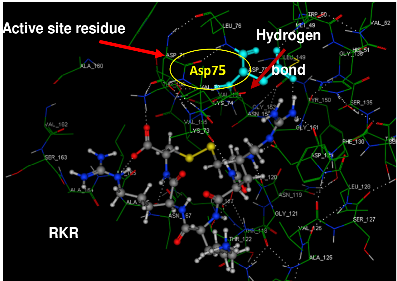
Figure 8. RKR-enzyme interaction after molecular dynamics at 300 K.
