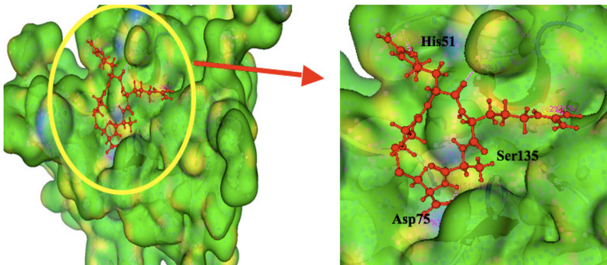
Figure 1. Hydrogen bond between RKR ligand and enzyme.
