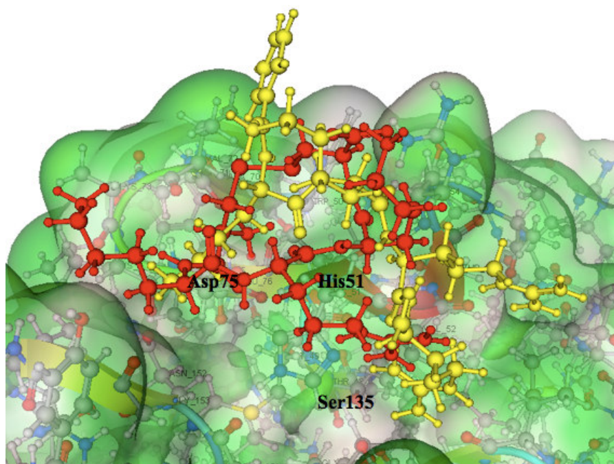
Figure 3. Superimpose result of RKR ligand (red) with standard ligand (yellow)
