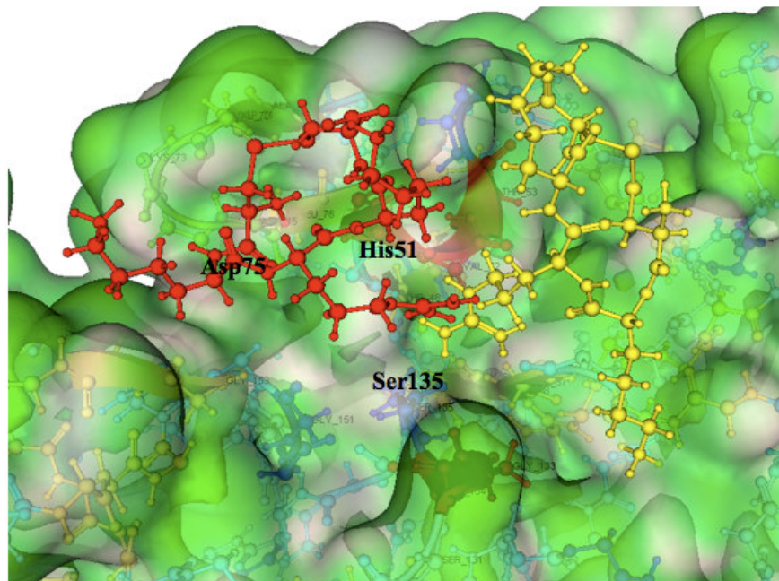
Figure 2. Superimpose result of RKR ligand (red) with KRK Ligand (yellow)
