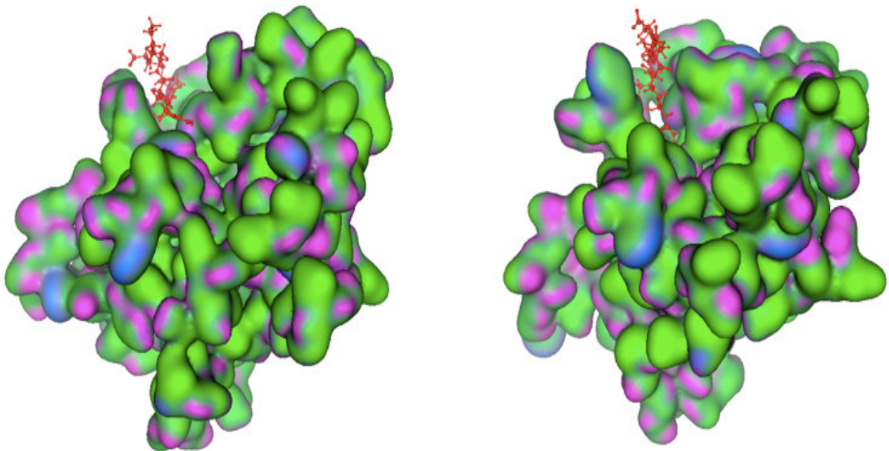
Figure 6. Protein-ligand conformation 50 and 75 ps.
