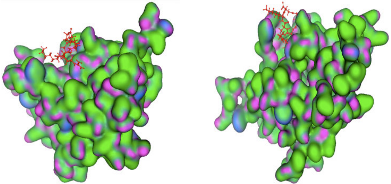
Figure 5. Protein-ligand conformation 0 and 25 ps.
