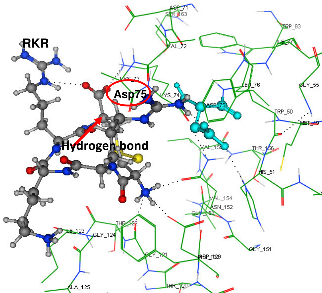
Figure 9. RKR-enzyme interaction after molecular dynamics at 312 K.
