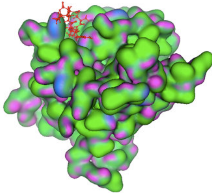
Figure 7. Protein-ligand conformation 100 ps.
