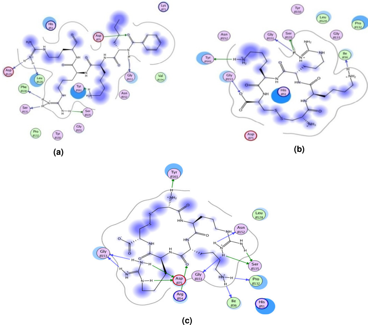
Figure 4. a) KRK; (b) RKR; (c) Standard ligand (Bz-Nle-K-R-R-H).
