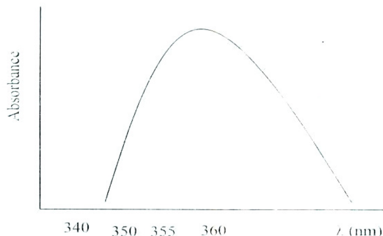
Figure 1. Absorption maxima for iron-oxine complex.
