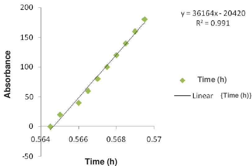
Figure 4. The stability curve of the proposed method.
