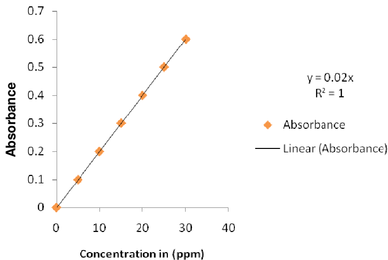
Figure 2. Calibration curve using oxine chloroform solution.
