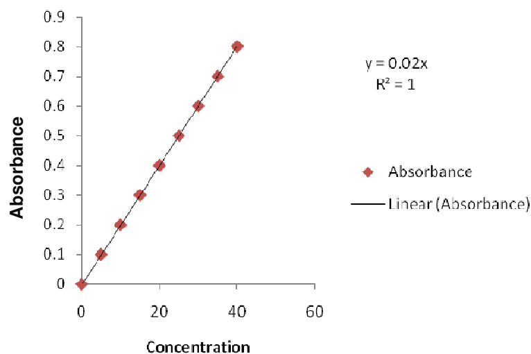
Figure 3. Calibration curve using oxine acidified reagent.
