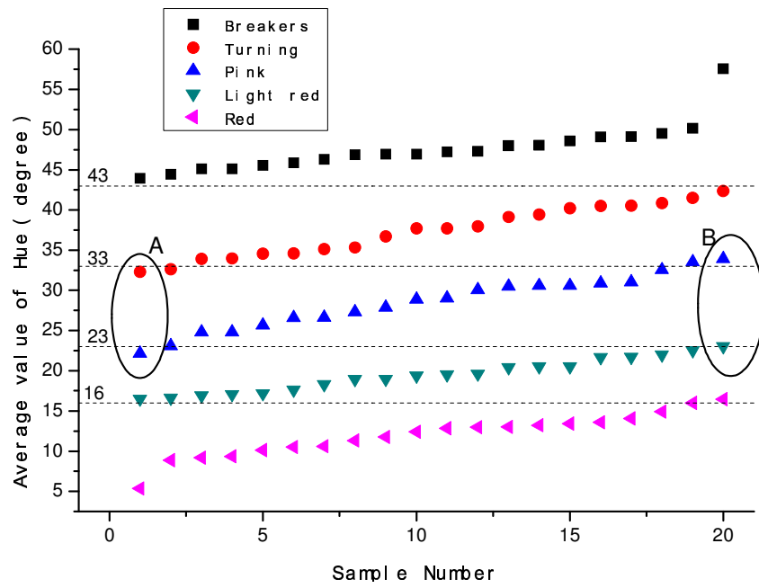
Figure 7. Distribution of hue average for fresh tomatoes.
