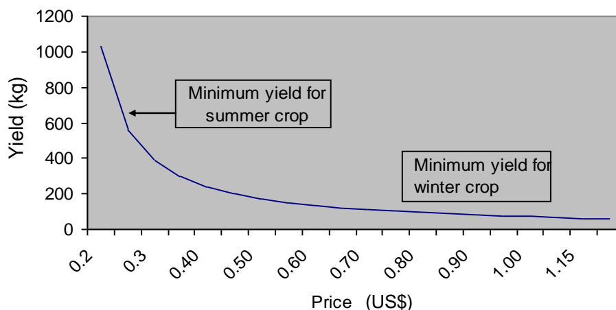
Figure 1. Minimum yield for given prices to break-even in cucumber production under greenhouse.
