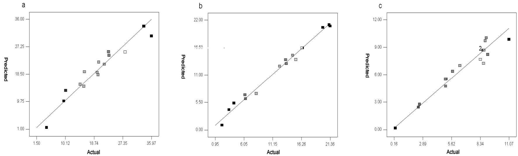
Figure 4. Plot of predicted versus actual values for lignocellulolysis. A, Plot of predicted versus actual lignin loss; B, plot of predicted versus actual hemicellulose loss; C, plot of predicted versus actual cellulose loss.
