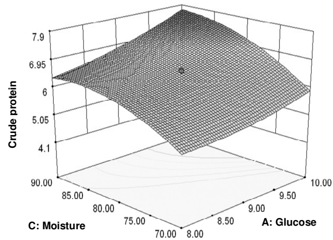
Figure 5. Response surface model graph for maximum crude protein content (A: glucose = 10 mg/g CS and C: moisture = 90%; hold value B: \text{CuSO}_4 = 4.5 \mu\text{M/g} CS).
