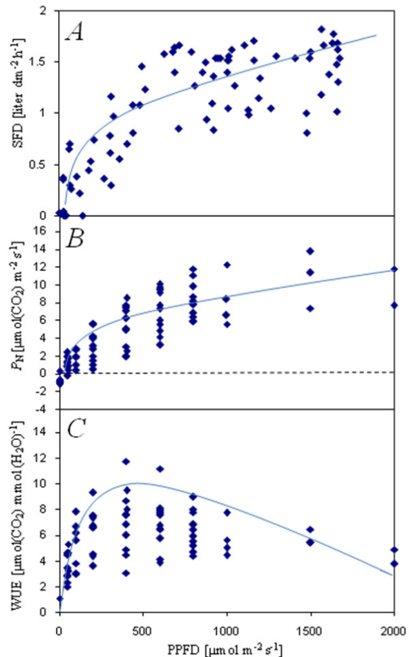
Figure 1. PPFD response curves of sap flow density (SFD) in Quercus suber grown in North Tunisia.
