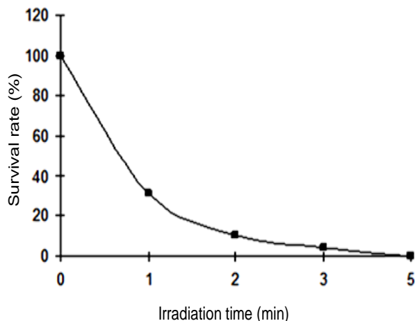
Figure 1. Effect of UV irradiation on survival of wild-type cells of Chlamydomonas reinhardtii CC-124.
