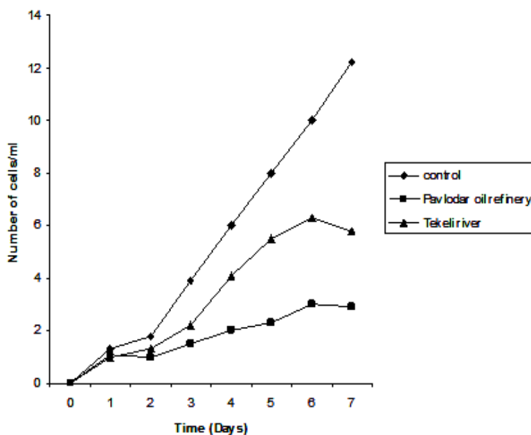
Figure 3. Effect of mutagenic activity of different types of polluted waters on survival pigmented mutant 124y-1.
