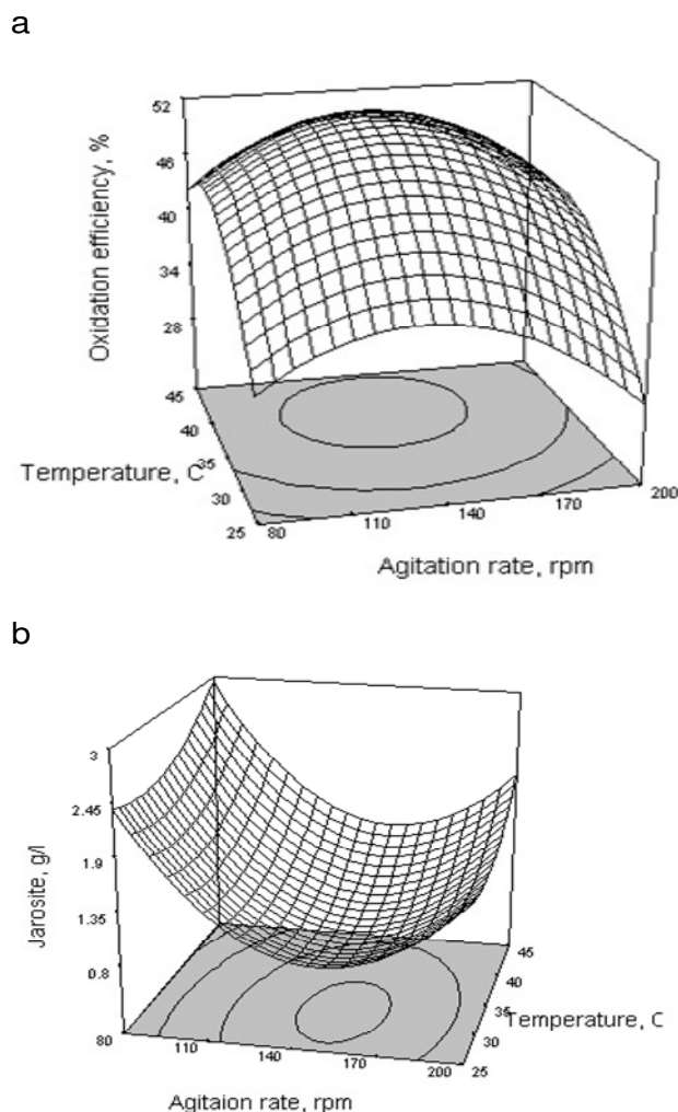
Figure 7. A 3D-response surface plot of the effect of agitation rate and temperature on (a) oxidation efficiency and (b) jarosite formation. The other variables were set at zero levels.
