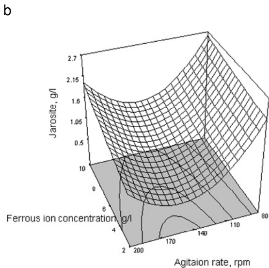
Figure 5. A 3D-response surface plot of the effect of Fe^{2+} ion concentration and agitation rate on (a) oxidation efficiency and (b) jarosite formation. The other variables were set at zero levels.
