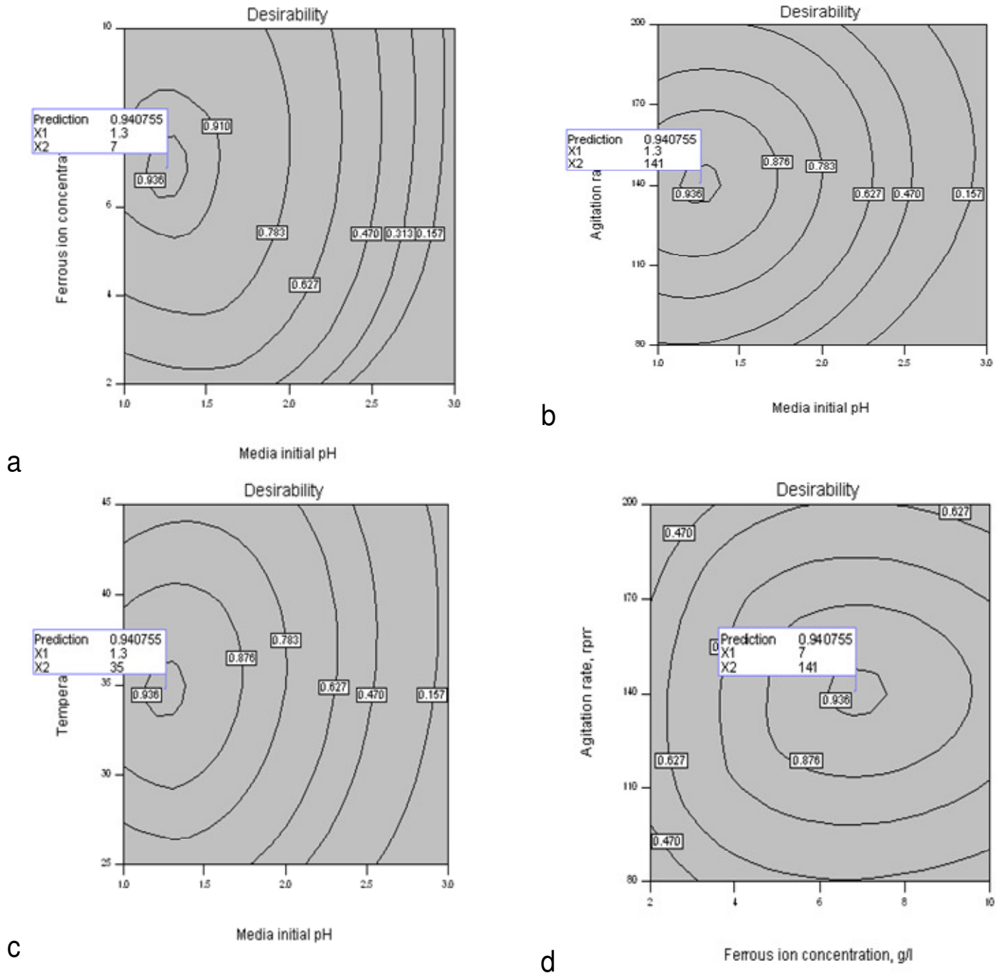
Figure 8. Desirability fitted surface for numerical optimization of the respective goals within the range of four factors of maximum oxidation efficiency and minimum amount of jarosite; (a), effect of media initial pH and Fe^{2+} ion concentration; (b) effect of media initial pH and agitation rate; (c) effect of media initial pH and temperature; (d), effect of agitation rate and Fe^{2+} ion concentration; (e), effect of temperature and Fe^{2+} ion concentration; (f), effect of temperature and agitation rate.
