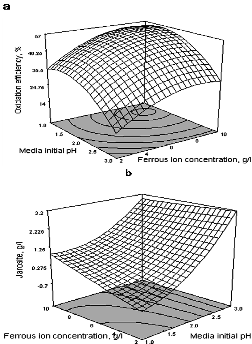
Figure 2. A 3D-response surface plot of the effect of media initial pH and \text{Fe}^{2+} ion concentration on (a) oxidation efficiency and (b) jarosite formation. The other variables were set at zero levels.
