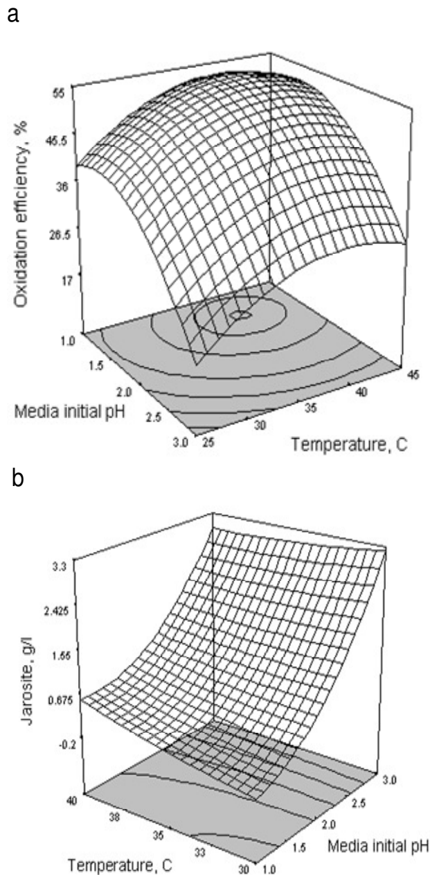
Figure 4. A 3D-response surface plot, of the effect of media initial pH and temperature on (a) oxidation efficiency (b) jarosite formation. The other variables were set at zero levels.
