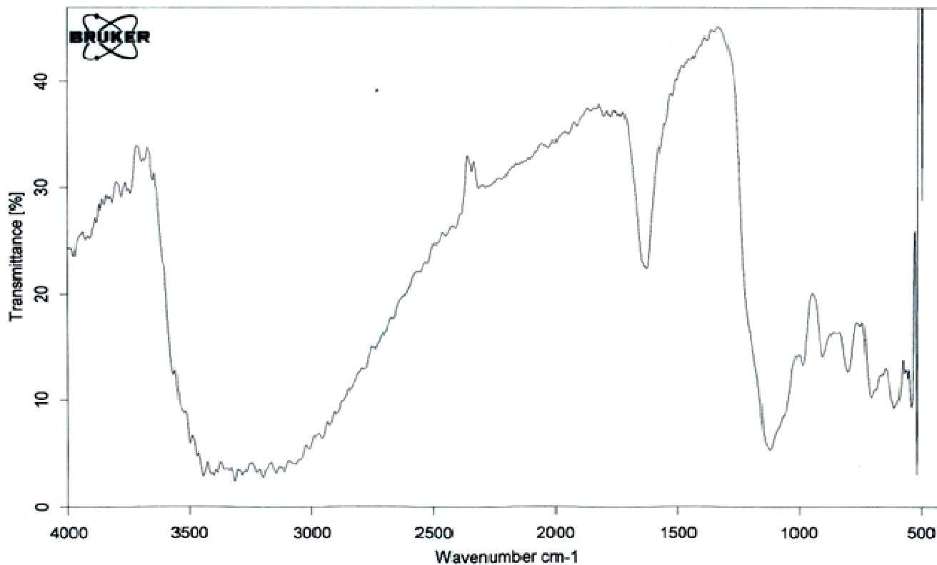
Figure 1. FTIR of iron precipitates mediated by the isolated microorganism from the hot spring.
