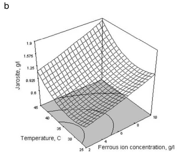
Figure 6. A 3D-response surface plot of the effect of Fe^{2+} ion concentration and temperature on (a) oxidation efficiency and (b) jarosite formation. The other variables were set at zero levels.
