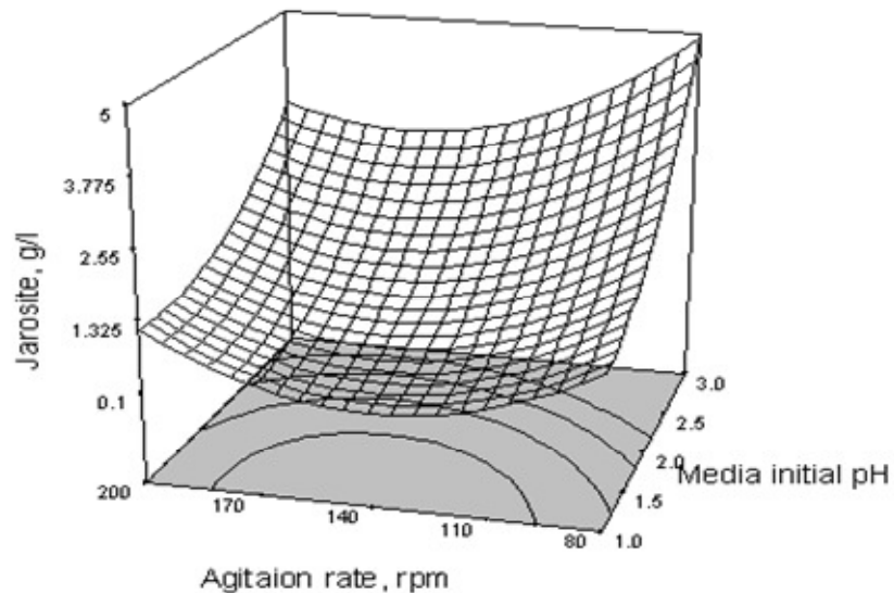
Figure 3. A 3D- response surface plot of the effect of the media initial pH and agitation rate on (a) oxidation efficiency (b) jarosite formation. The other variables were set at zero levels.
