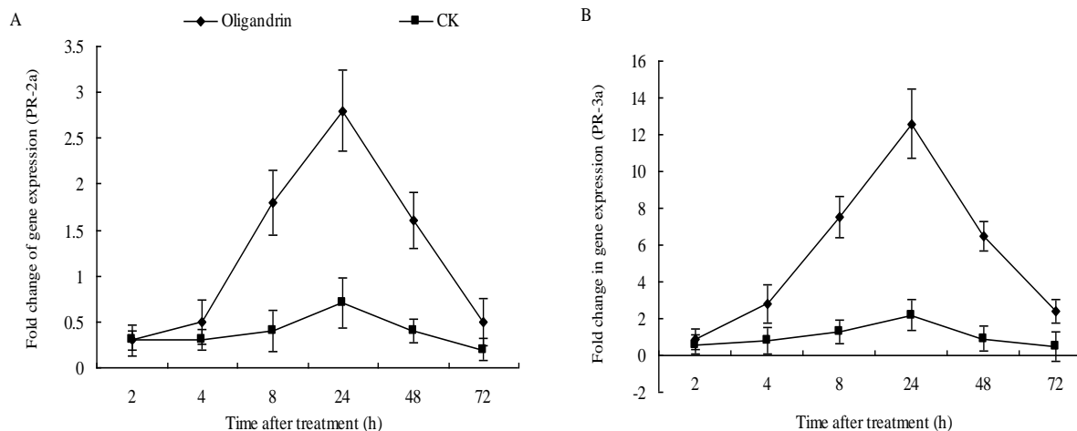
Figure 3. Induction of defense gene. A, PR-2a (extracellular \beta -1, 3-glucanase); B, PR-3a (extracellular chitinase) expression by oligandrin in tomato fruit at 2, 4, 8, 24, 48 and 72 h (method of 2^{-\Delta\Delta Ct} ). Bars represent standard deviations of the means.
