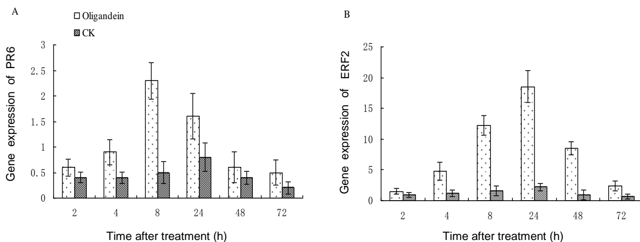
Figure 4. The defense gene (A is PR6 and B is ERF2) expression in tomato fruits induced by oligandrin at 2, 4, 8, 24, 48 and 72 h (method of 2^{-\Delta\Delta Ct} ).
