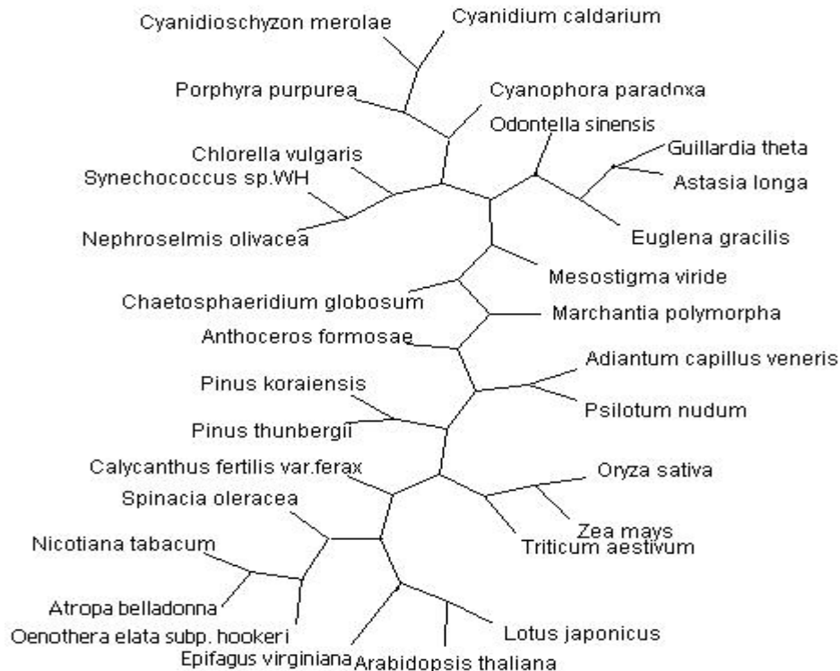
Figure 4. Network tree of common genes in complete chloroplast genomes. The poales are closely placed in a common clade while unrelated species such as C. vulgaris is in a clade of green algae. Generating a good tree is important in predicting gene function based on evolutionary distance.
