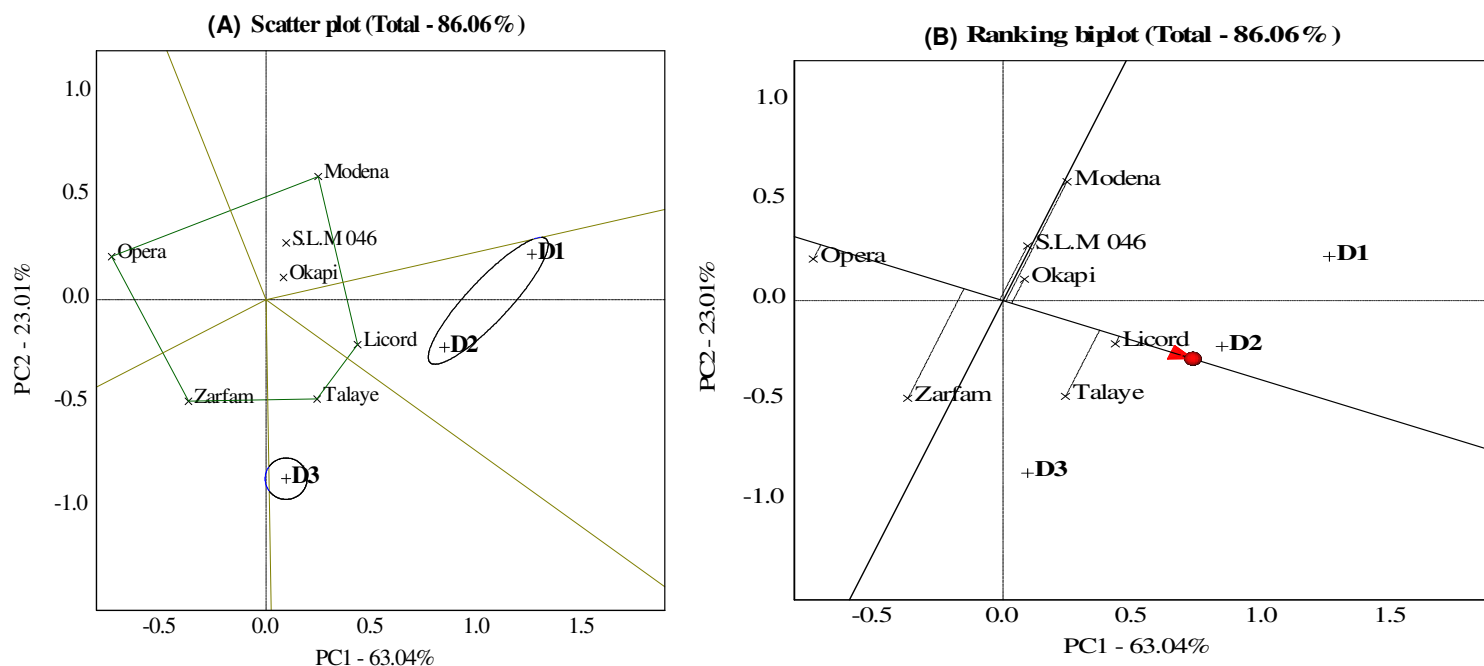
Figure 4. The Biplot diagram of yield stability analysis of seven rapeseed cultivars (Licord, Okapi, Opera, S.L.M.046, Zarfam, Modena, and Talaye) using GGE biplot method. A- Scatter plot of cultivars based on relative advantage in the experimental units (different levels of drought stress, D1, D2, and D3). B- Ranking Biplot of cultivars based on mean yield and yield stability in the studied experimental units.
