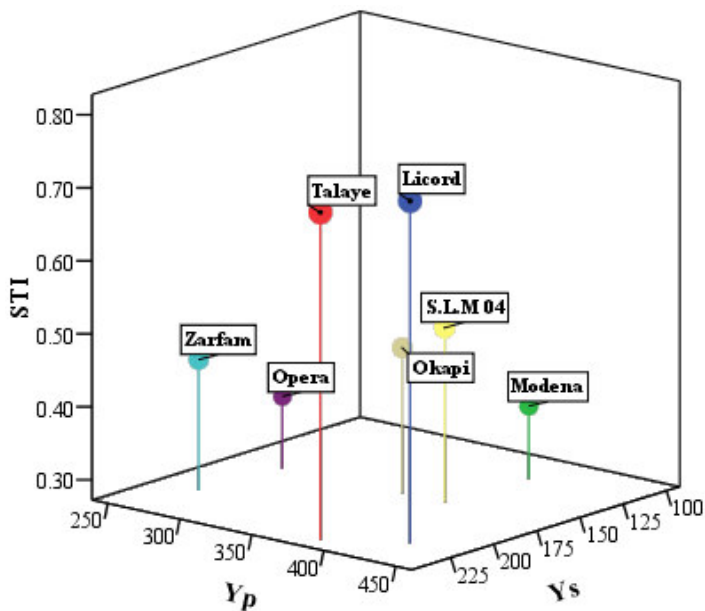
Figure 2. 3D scatter plot of studied cultivars based on mean yield under irrigation ( Y_p ), mean yield under stress conditions ( Y_s ) and stress tolerance index (STI).
