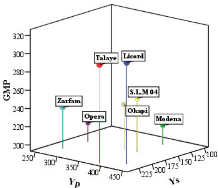
Figure 3. 3D scatter plot of studied cultivars based on mean yield under irrigation ( Y_p : yield potential), mean yield under stress condition ( Y_s ) and geometric mean productivity (GMP).
