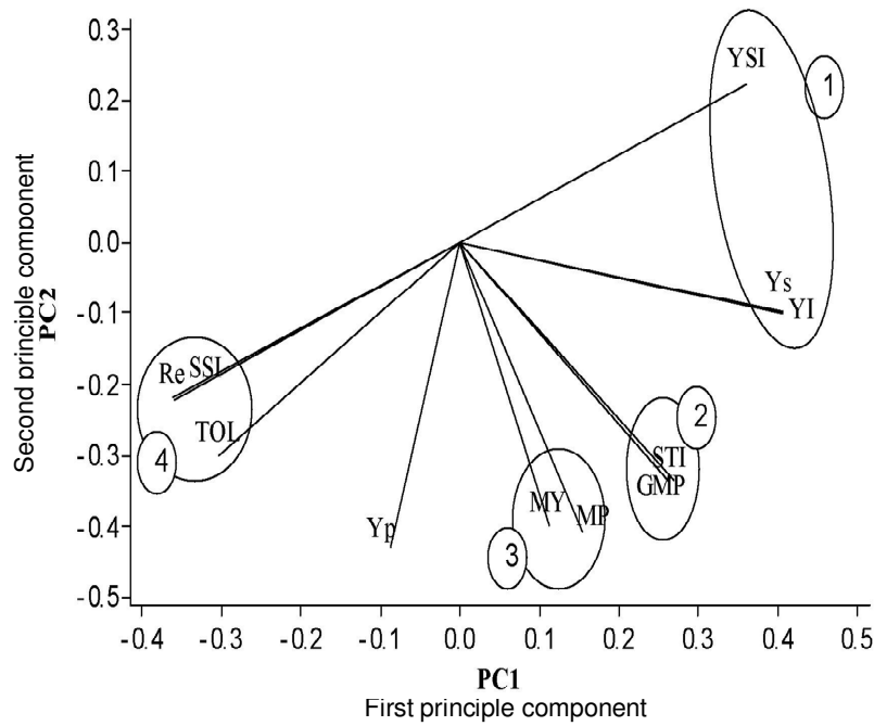
Figure 1. The biplot diagram of principle components analysis of 7 cultivars of winter rapeseed according to mean measured indices together with mean seed yield under stress ( Y_s ) and irrigation ( Y_p ) conditions. Re: % reduction; STI: stress tolerance index; GMP: geometric mean productivity; SSI: stress susceptibility index; YSI: yield stability index; MP: mean productivity; TOL: tolerance index; YI: yield index; MY: mean yield.
