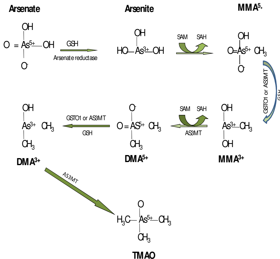
Figure 1. Arsenic metabolism showing arsenate reduction to arsenite and methylation to pentavalent (MMA 5+ , DMA 5+ ) and trivalent (MMA 3+ , DMA 3+ ) forms.
