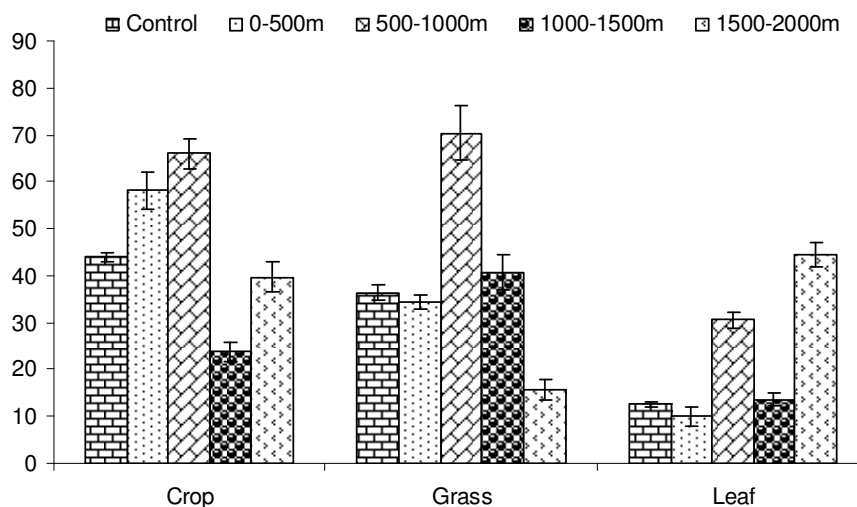
Figure 4. Variation in fluoride (mg/kg) content in Crop, Grass and Leaf samples in control and experimental site (Mean \pm SD).
