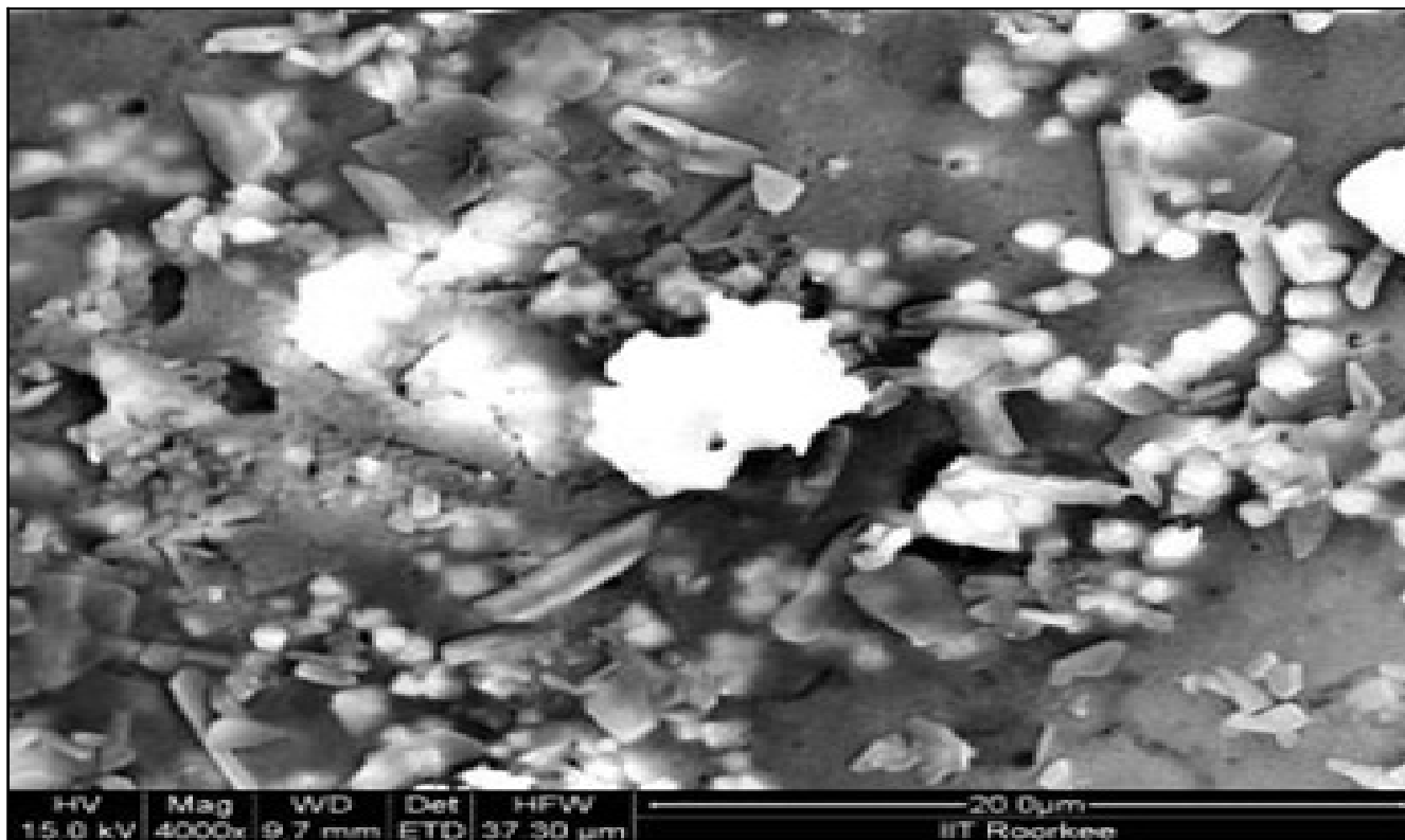
Figure 2. Scanning electron micrograph of tea waste biomass.
