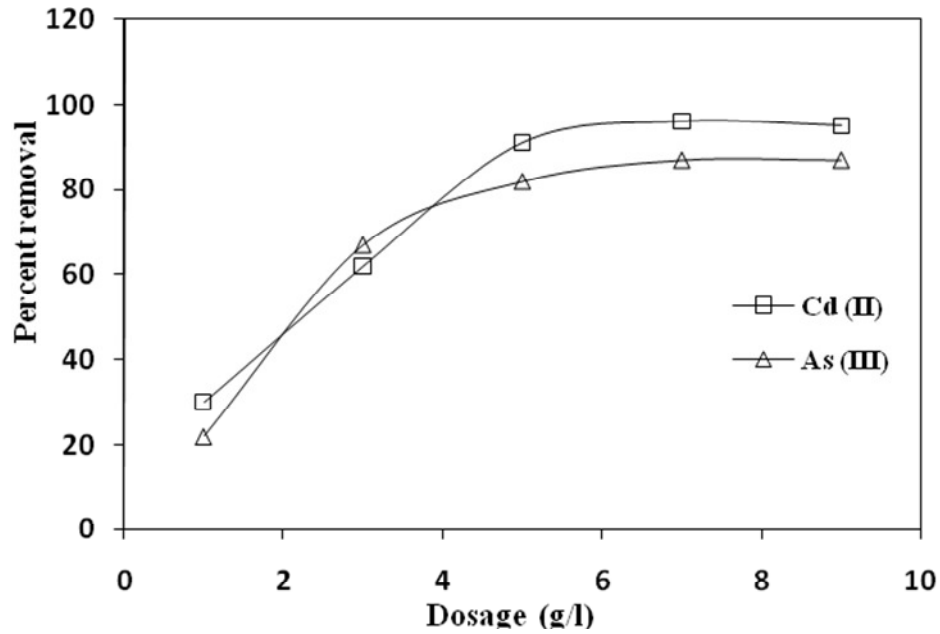
Figure 5. Effect of dosage on the biosorption of metal ions.
