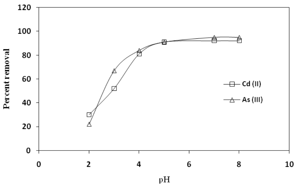
Figure 4. Effect of pH on the biosorption of metal ions onto tea waste biomass.
