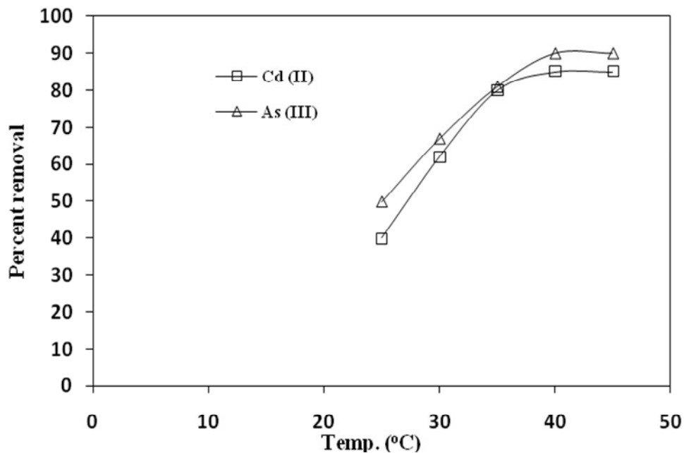
Figure 6. Effect of temperature onto the removal of metal ions at pH 5.5 and pH 7.5.
