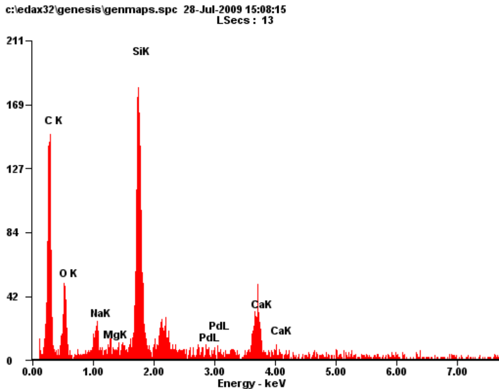
Figure 1. EDX analysis of tea waste biomass.
