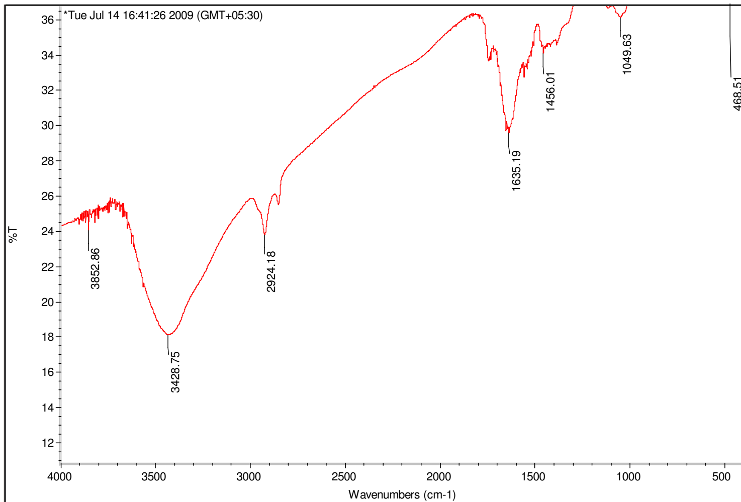
Figure 3. Fourier transform infrared (FTIR) spectrum of tea waste biomass in a KBr disc.
