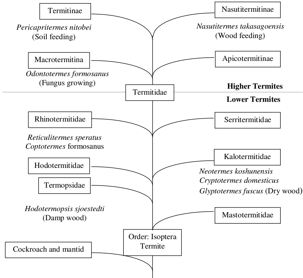
Figure 1. Flow diagram of phylogeny of termite family (Ohkuma et al., 2001).
