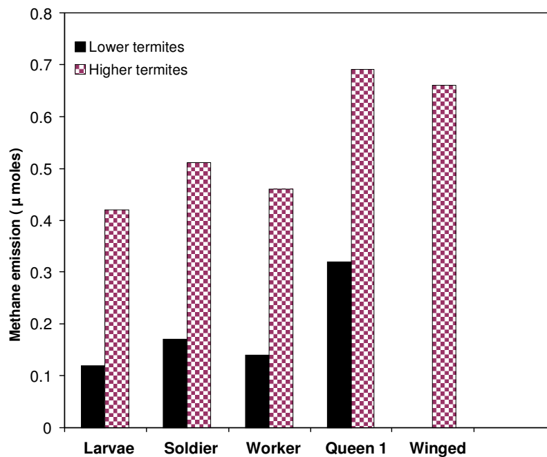
Figure 3. Emission of methane in situ by different castes of termites.
