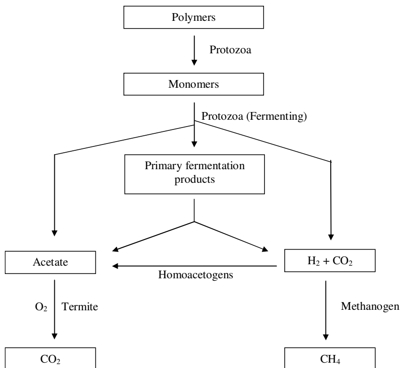
Figure 2. Fermentation of polymers in the termite guts (Tholen et al., 1997).
