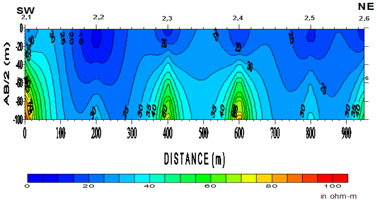
Figure 10. The pseudosection for profile 2 of Odo Ara study area.
