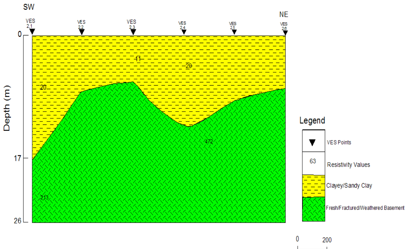
Figure 14. The geoelectric section for profile 2 of the study area.
