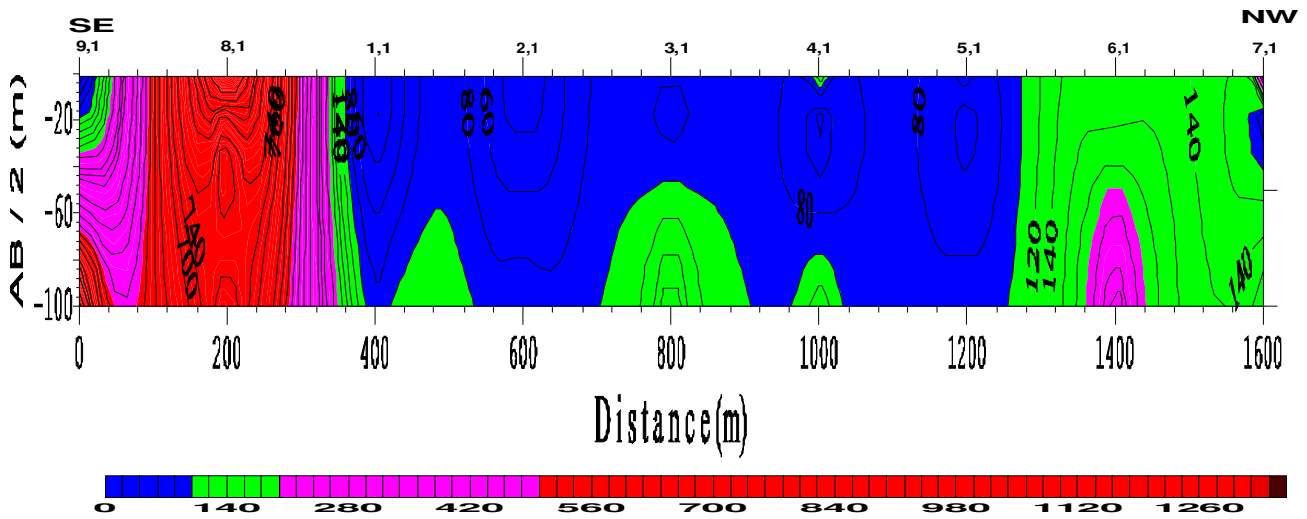
Figure 12. The pseudosection for section 1 of Odo Ara study area.
