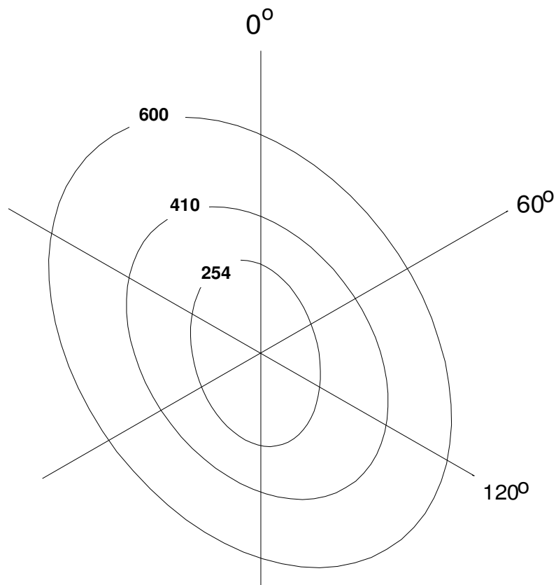
Figure 18. The anisotropy polygon of station 9,2 of the study area.
