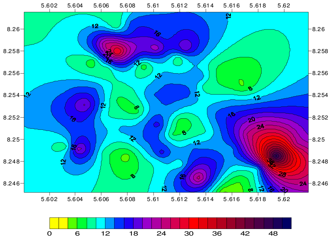
Figure 7. The isopach map of the overburden in the study area.
