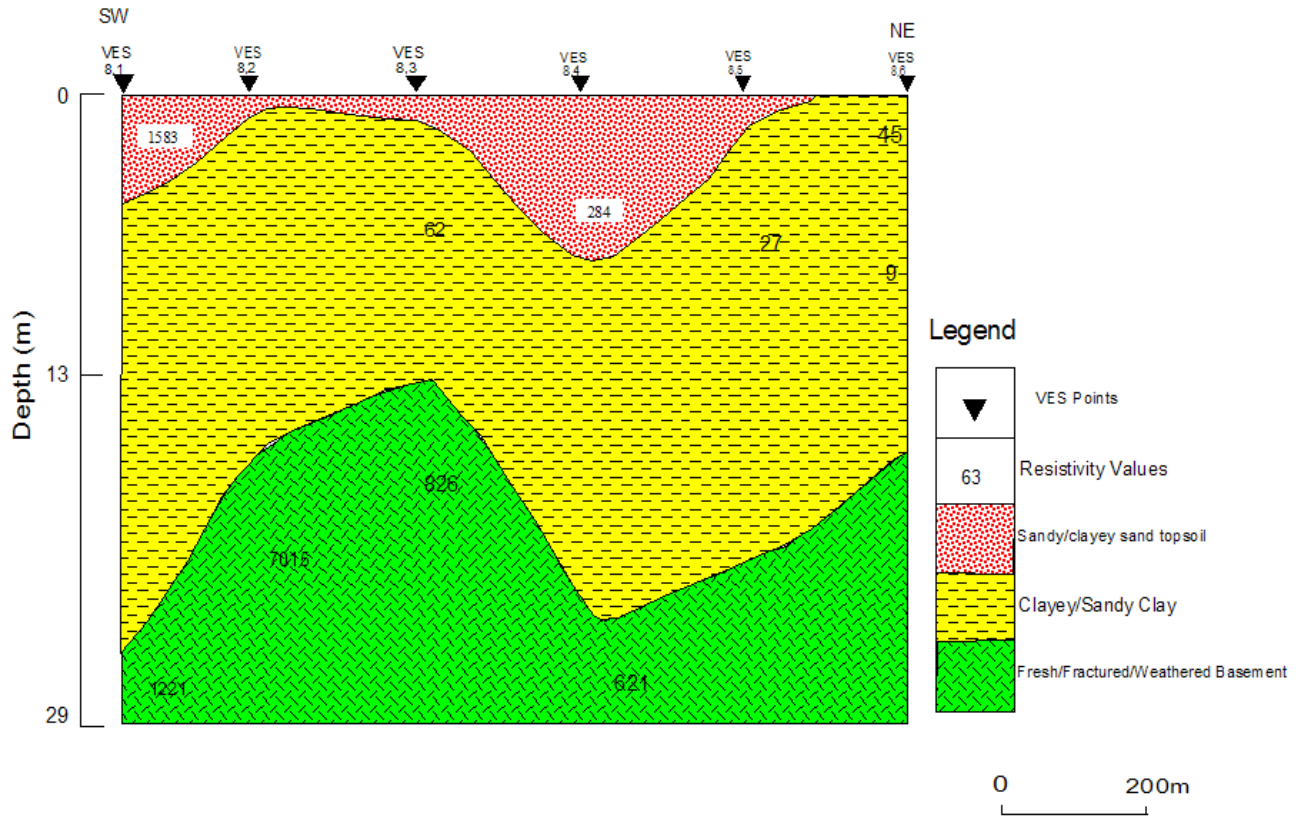
Figure 15. The geoelectric section for profile 8 of the study area.
