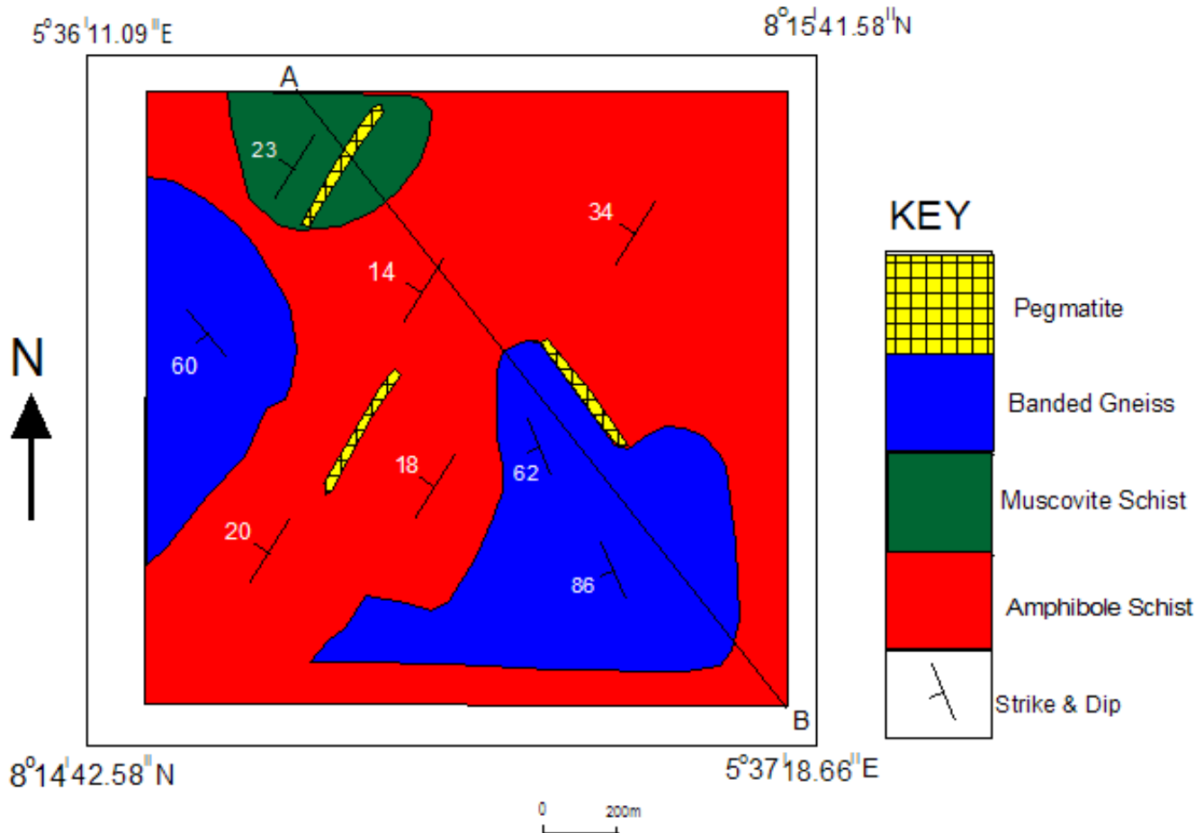
Figure 2. The geological map of Odo Ara area.
