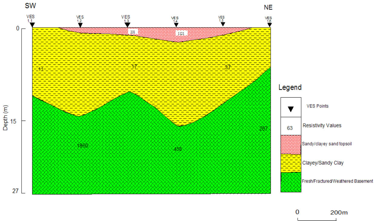
Figure 13. The geoelectric section for profile 1 of the study area.
