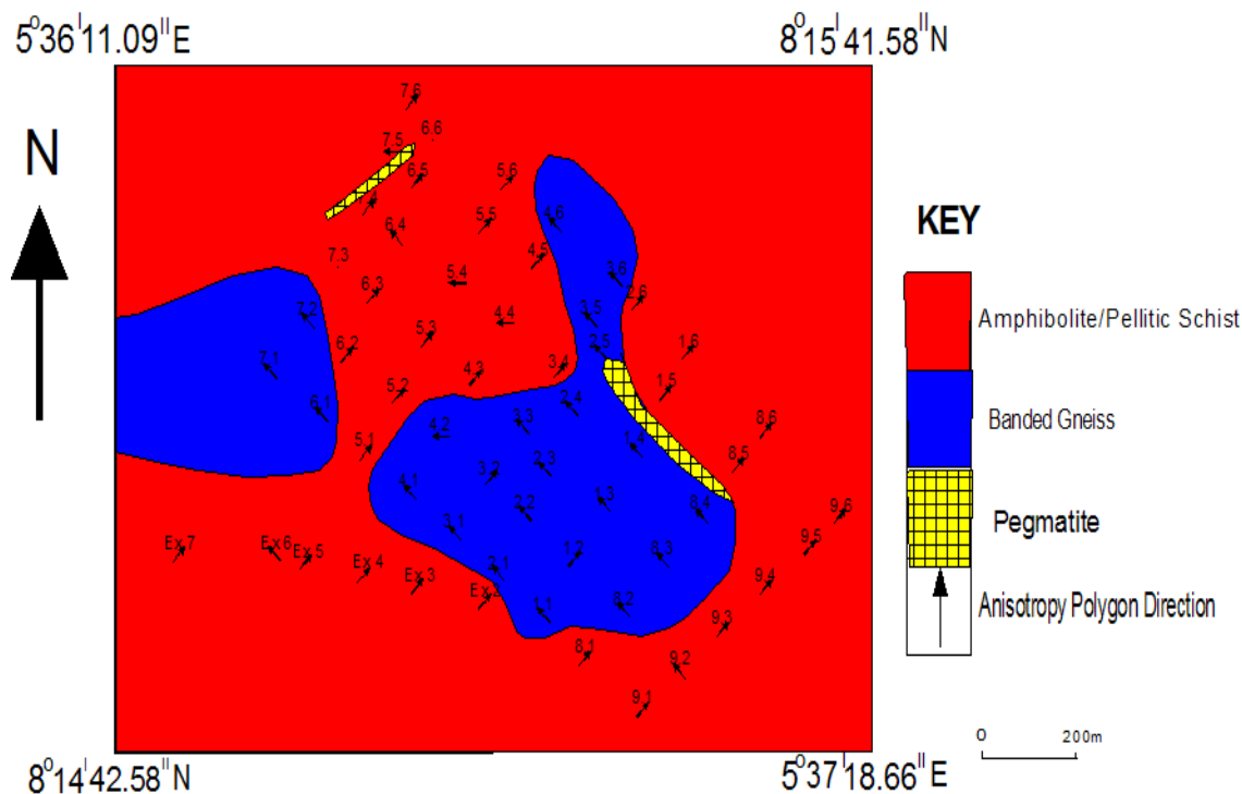
Figure 19. The geological map produced from the superposition of the anisotropy directions and the resistivity map of Odo Ara.
