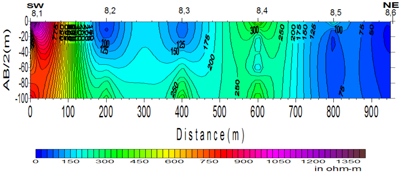
Figure 11. The pseudosection for profile 8 of Odo Ara study area.
