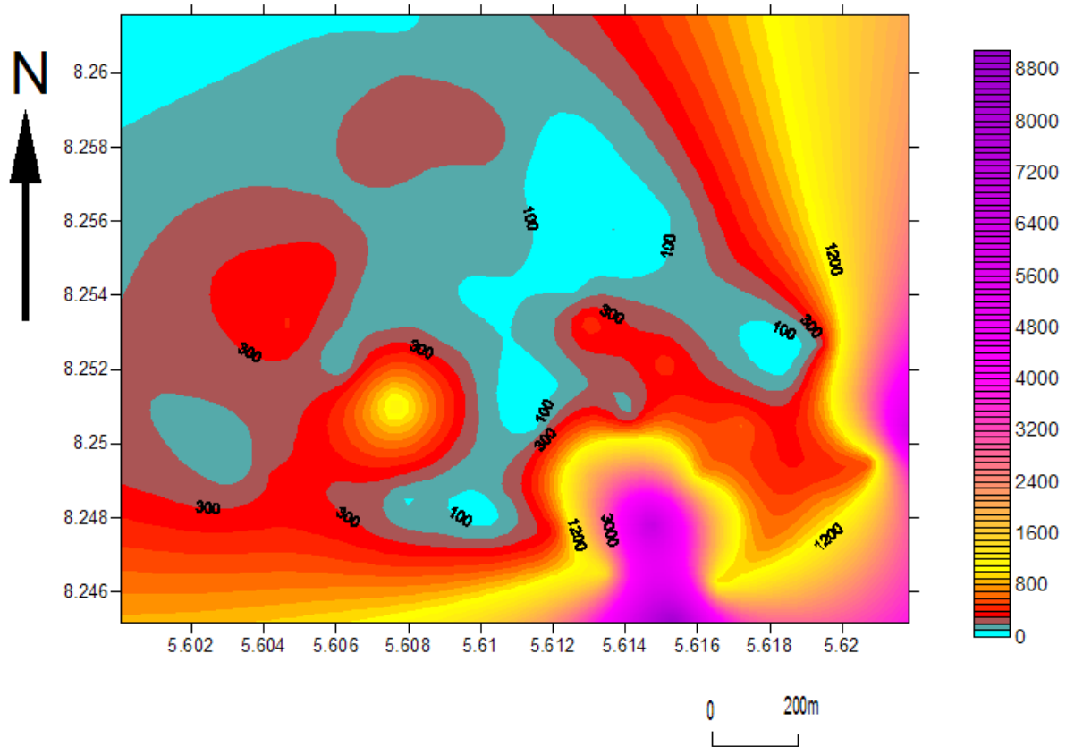
Figure 8. The iso-resistivity map of the study area produced from the iterated resistivity data.
