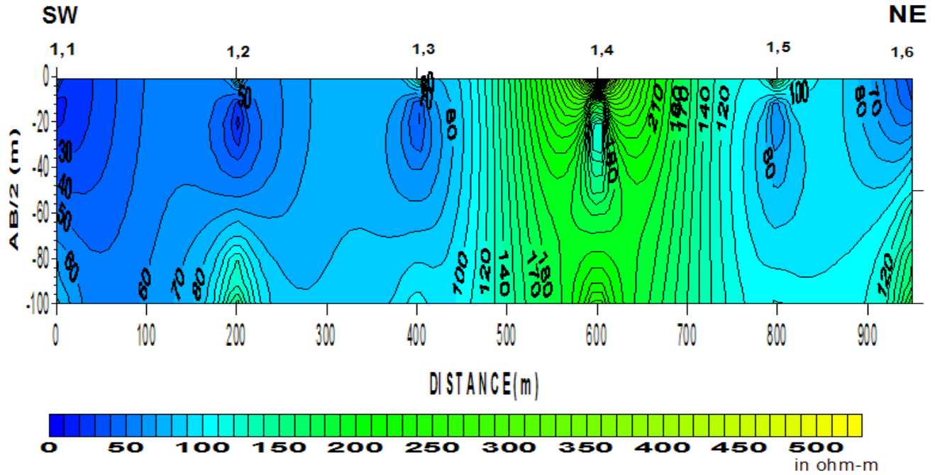
Figure 9. The pseudosection for profile 1 of Odo Ara study area.
