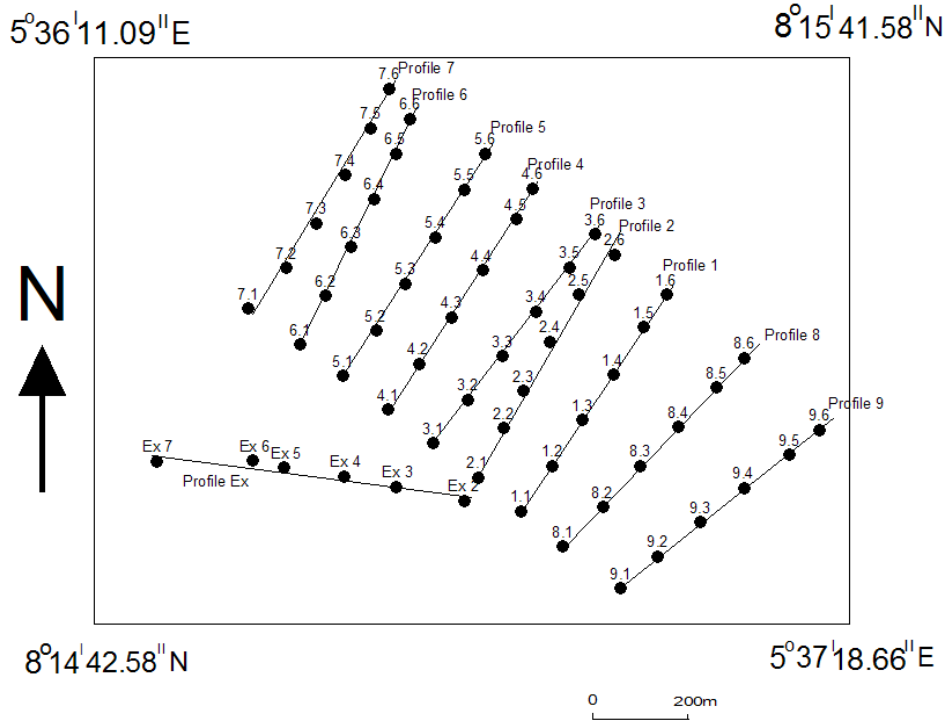
Figure 4. The layout of Odo Ara RVES survey points.
