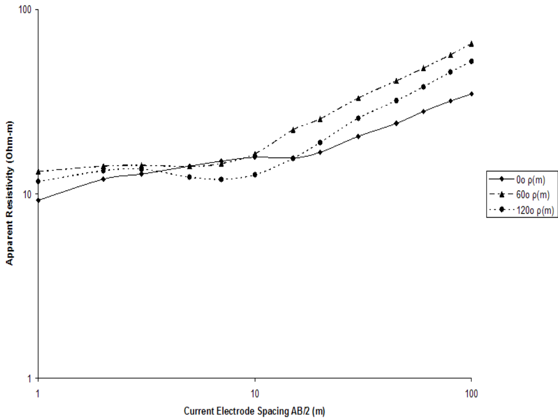
Figure 5. Typical RVES curve of Station 4,6 in the study area.
