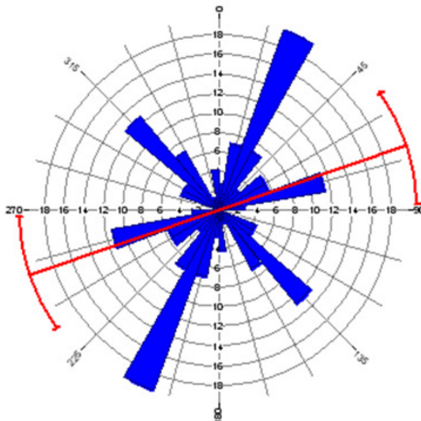
Figure 3. The rose diagram of the foliations of Odo Ara study area.
