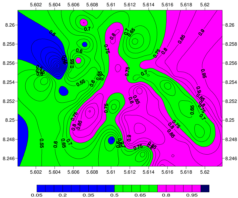
Figure 16. The reflection coefficient map of the study area.
