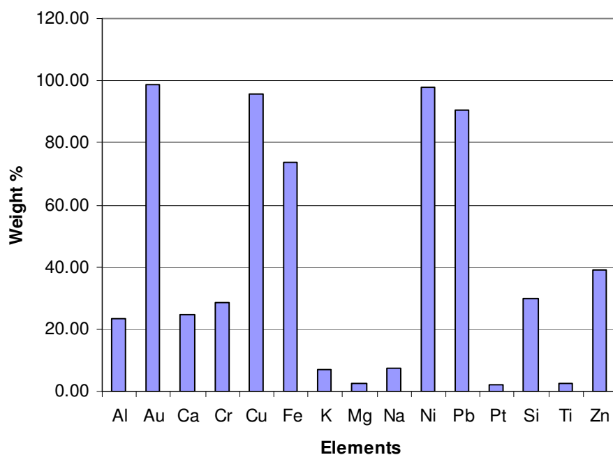
Figure 5. The graph showing the maximum amount of each element in the particles.
