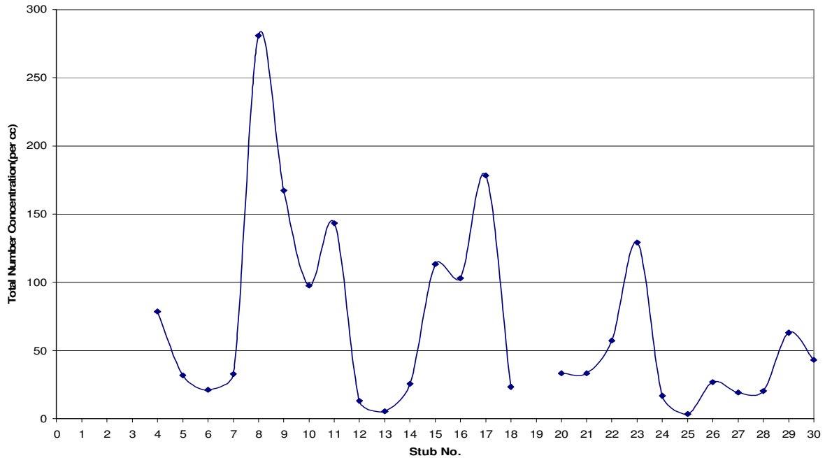
Figure 6. Variation of total number concentration of aerosols larger than 0.3µm in each stub observed.
