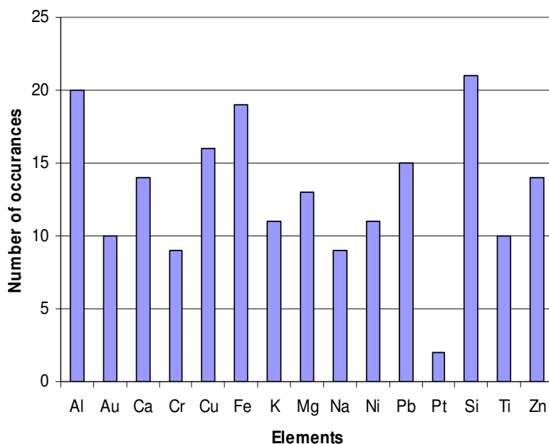
Figure 4. The graph showing the number of occurrences of elements.
