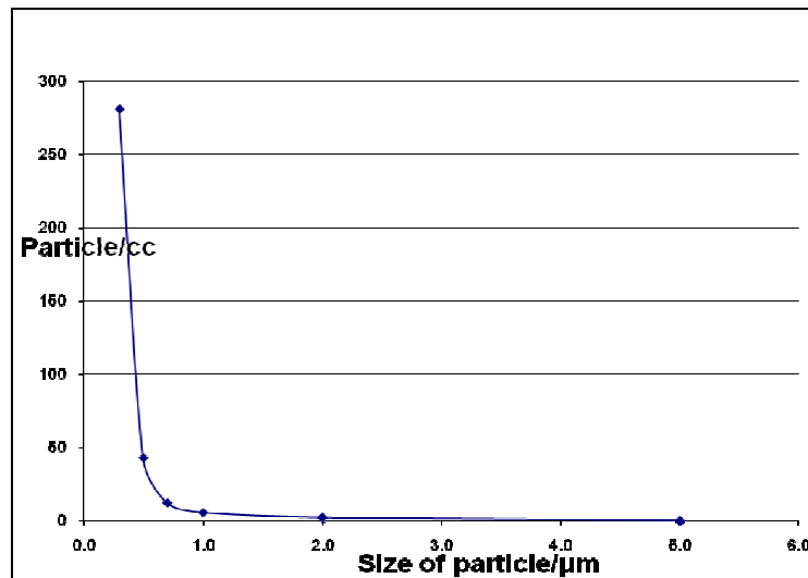
Figure 7. Particle concentration on 27 March, 2006.
