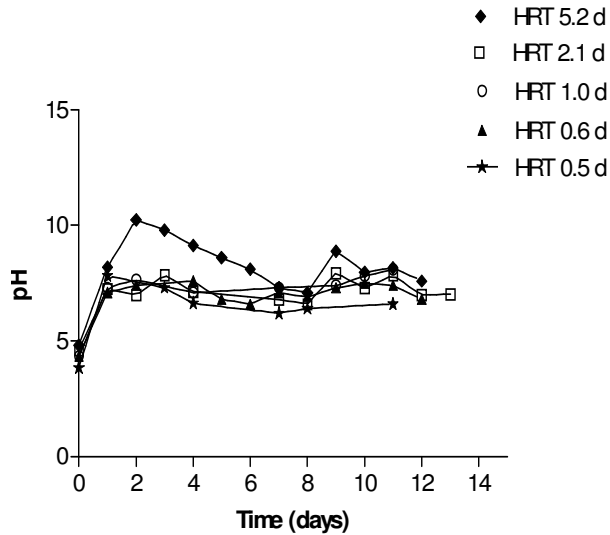
Figure 4. The pH changes during anaerobic treatment of potato-processing wastewater at 37°C using an UASB reactor at various HRTs.
