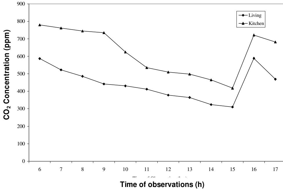
Figure 4. Observed CO 2 concentrations in low cost house.
