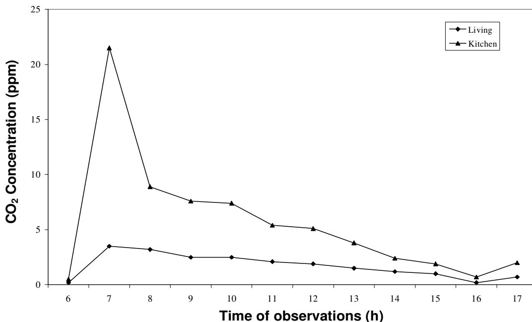
Figure 3. Observed CO 2 concentrations in low cost house
