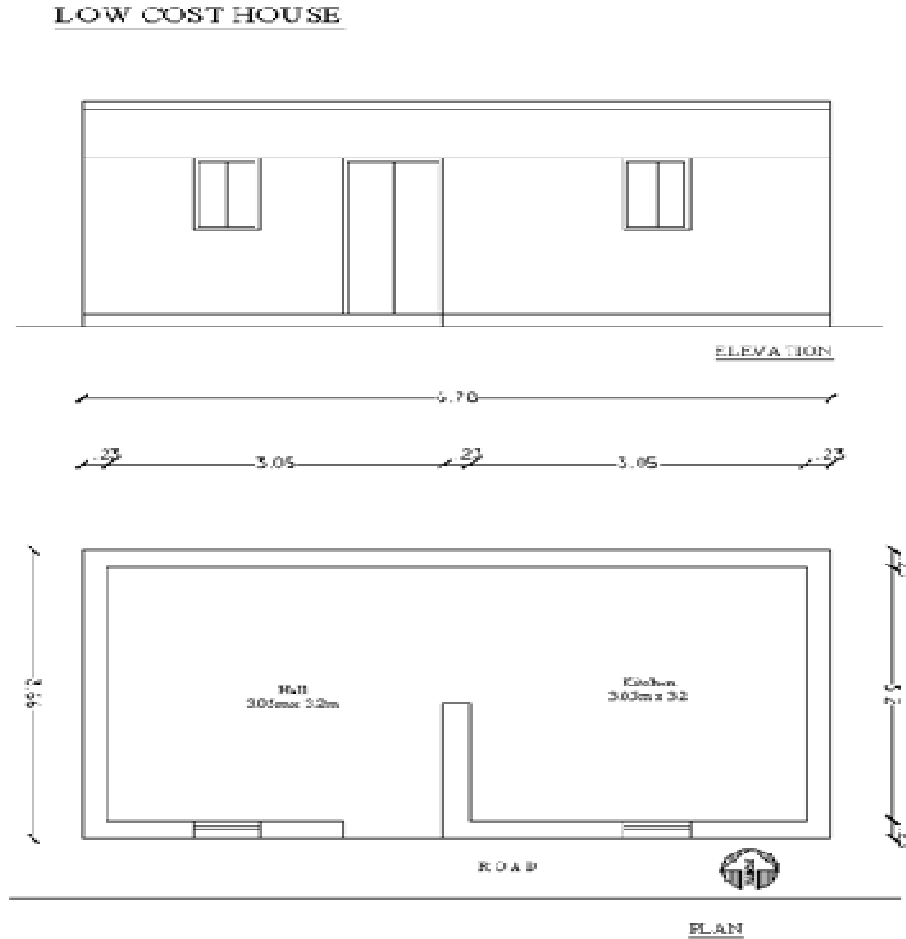
Figure 2. Plan and elevation of low cost house.
