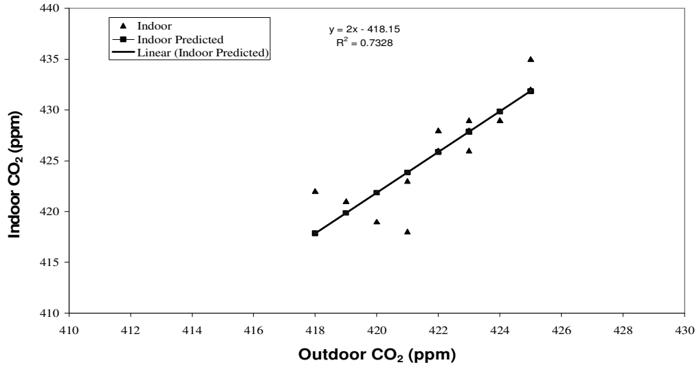
Figure 10. Indoor and outdoor relationship in kitchen for CO 2 in the green house.
