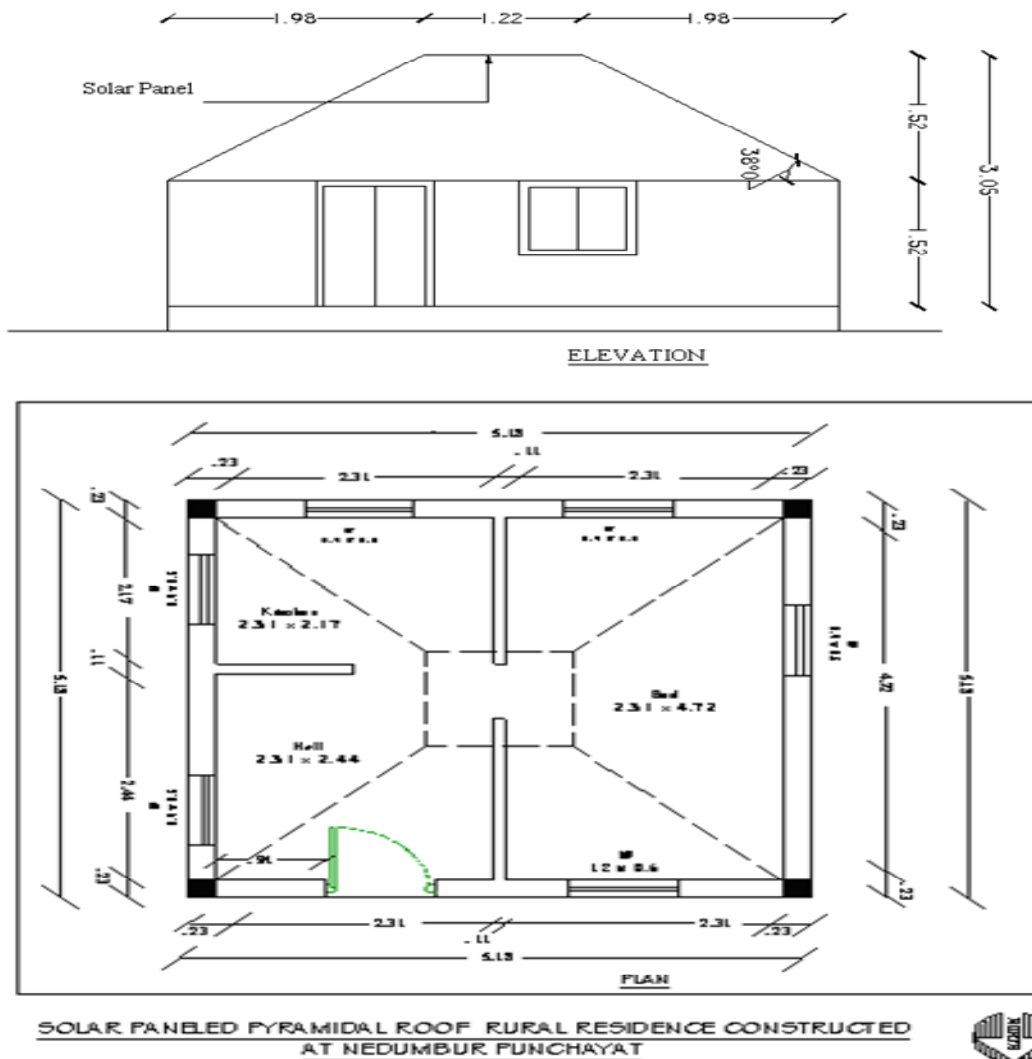
Figure 1. Plan and elevation of green house.
