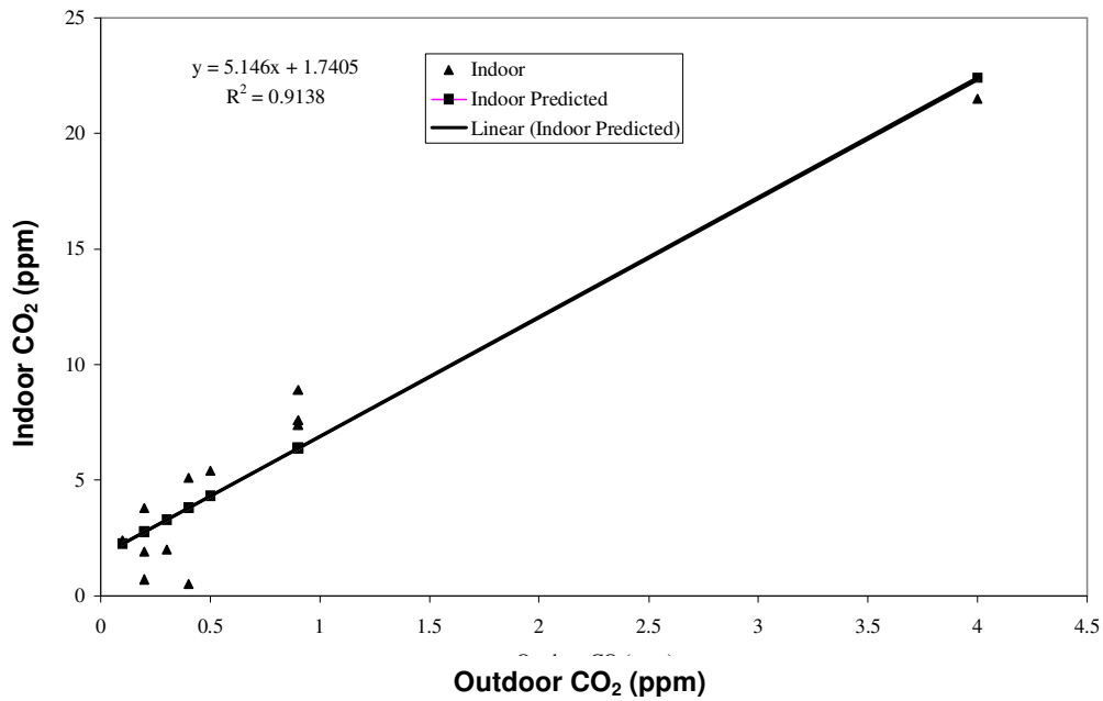
Figure 5. Relationships between indoor and outdoor concentration of co in kitchen at low cost house.
