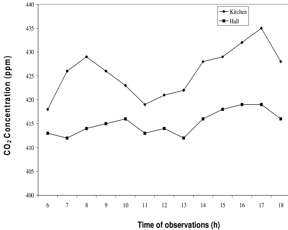
Figure 8. Observed indoor concentration of co 2 in the green house.
