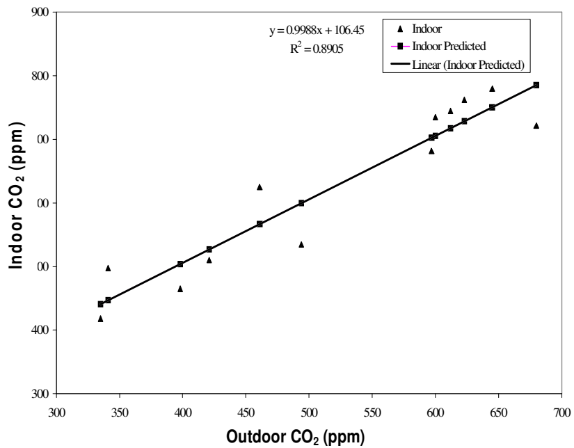
Figure 6. Relationships between indoor and outdoor concentration of co 2 in kitchen at low cost house.
