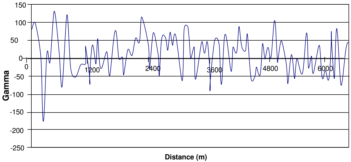
Figure 3a. Total relative magnetic intensity along traverse 11 (SE - NW) of the study area.
