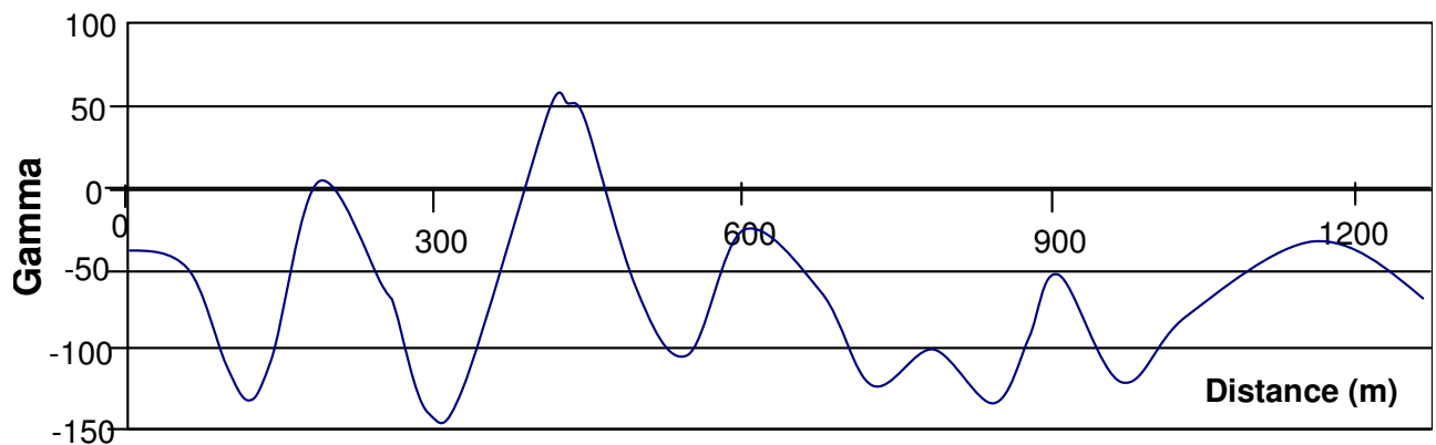
Figure 3c. Total relative magnetic intensity along traverse 14 (SE - NW) of the study area.
