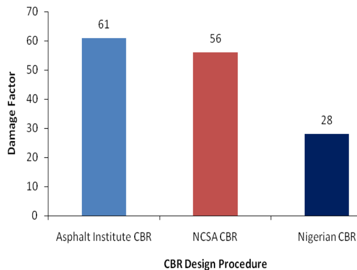
Figure 4b. CBR methods and rutting damage factors – Asphalt institute model (1982).
