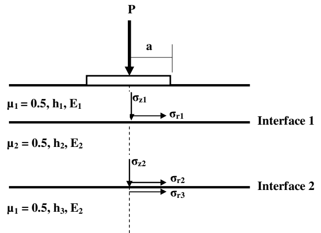
Figure 1. Three –layer pavement system showing location of stresses
