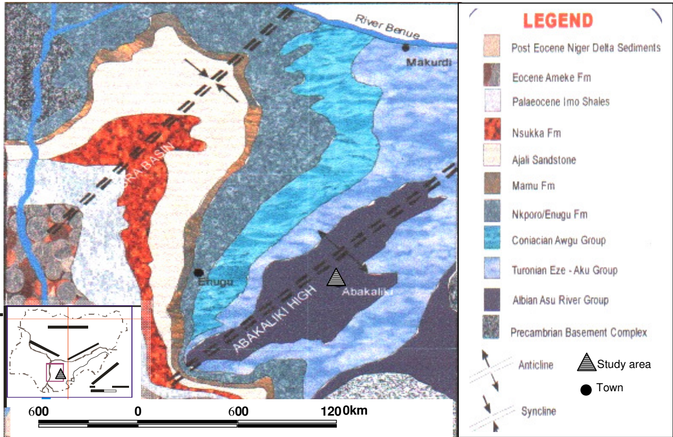
Figure 2. Generalized Geological map of southeastern showing the distribution of the Asu River Group and other lithologic units (Modified after Okogbue and Aghamelu, 2010a).
