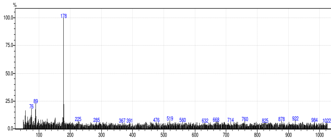
b. Anthracene [Retention time (RT) 9.670, m/z identification ion-178]
