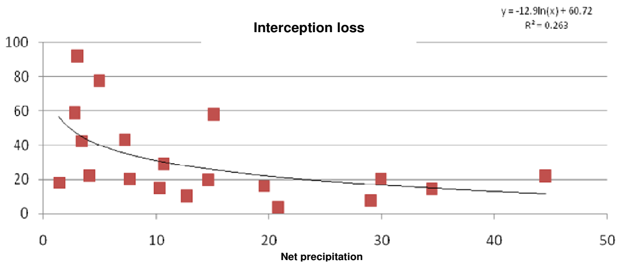
Figure 8. Regression of interception loss against rainfall (Leuceana).
