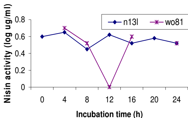
Figure 1. Effect of incubation time on nisin concentration (30°C) of two L. lactis strains over a 24 h fermentation period.
